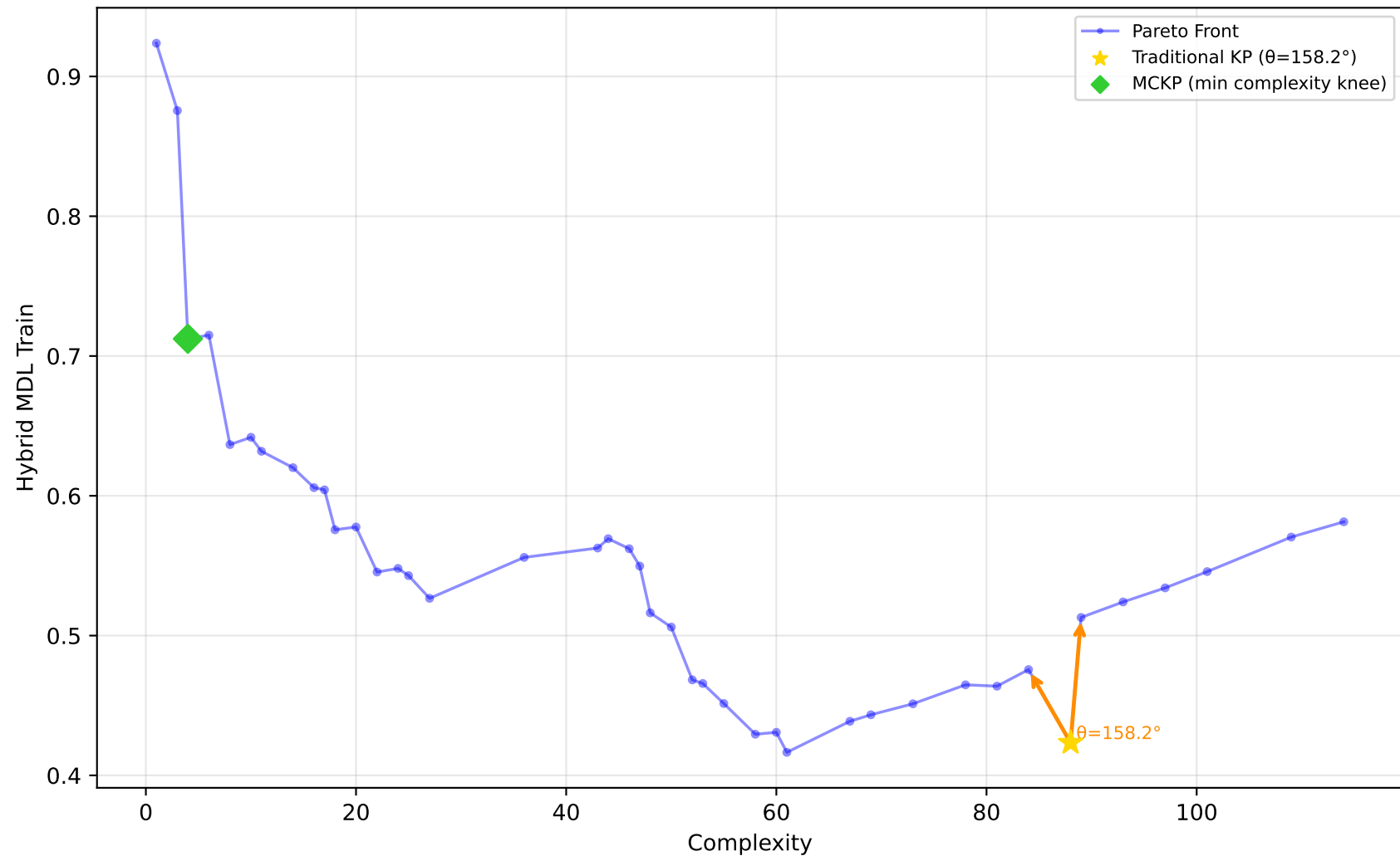
589_fri_c2_1000_25 - Run 22 - MVP - Hybrid MDL Train \lambda_1=0.00, \lambda_2=0.00, \lambda_3=0.00 | Difficulty: 1.00 | Method: hmr
