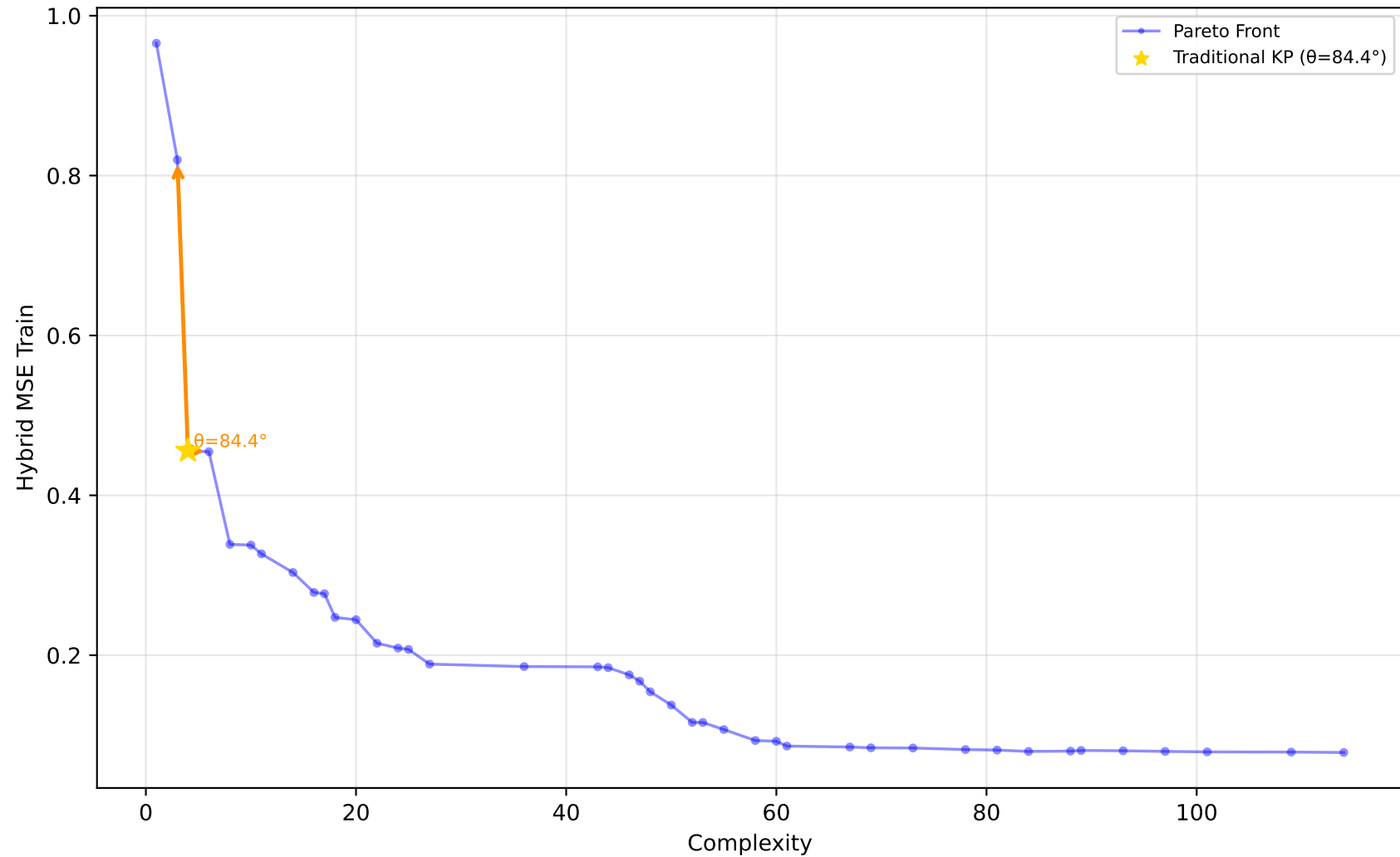
589_fri_c2_1000_25 - Run 22 - MVP - Hybrid MSE Train \lambda_1=0.30, \lambda_2=0.00, \lambda_3=0.20 | Difficulty: 1.00 | Method: hmr
