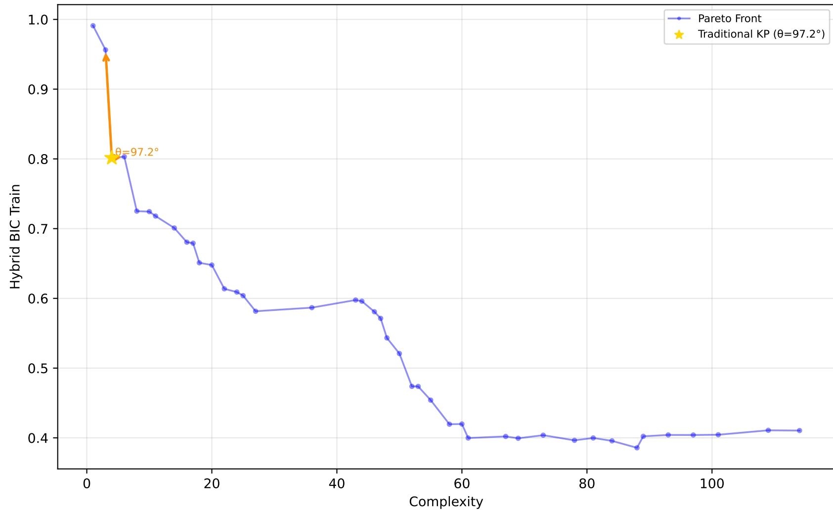
589_fri_c2_1000_25 - Run 22 - SVP - Hybrid BIC Train \lambda_1=0.20, \bar{\lambda}_2=0.00, \bar{\lambda}_3=1.00 | Difficulty: 1.00 | Method: hmr
