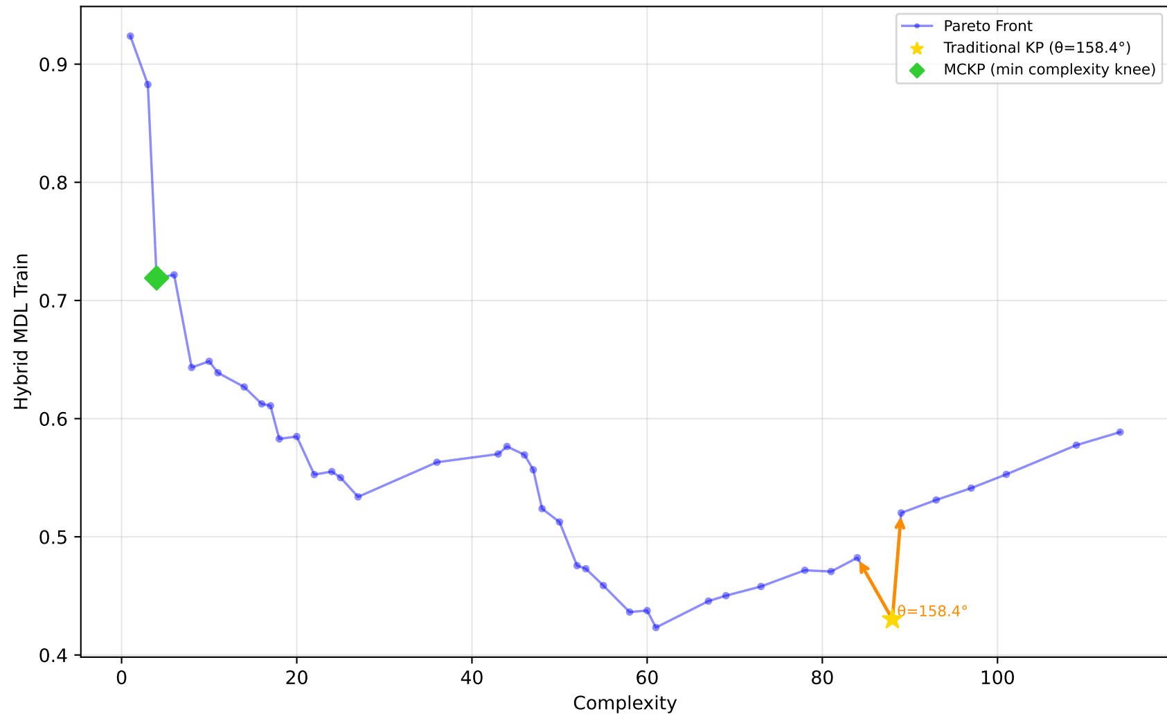
589_fri_c2_1000_25 - Run 22 - SVP - Hybrid MDL Train \lambda_1=0.10, \lambda_2=0.00, \lambda_3=0.10 | Difficulty: 1.00 | Method: hmr
