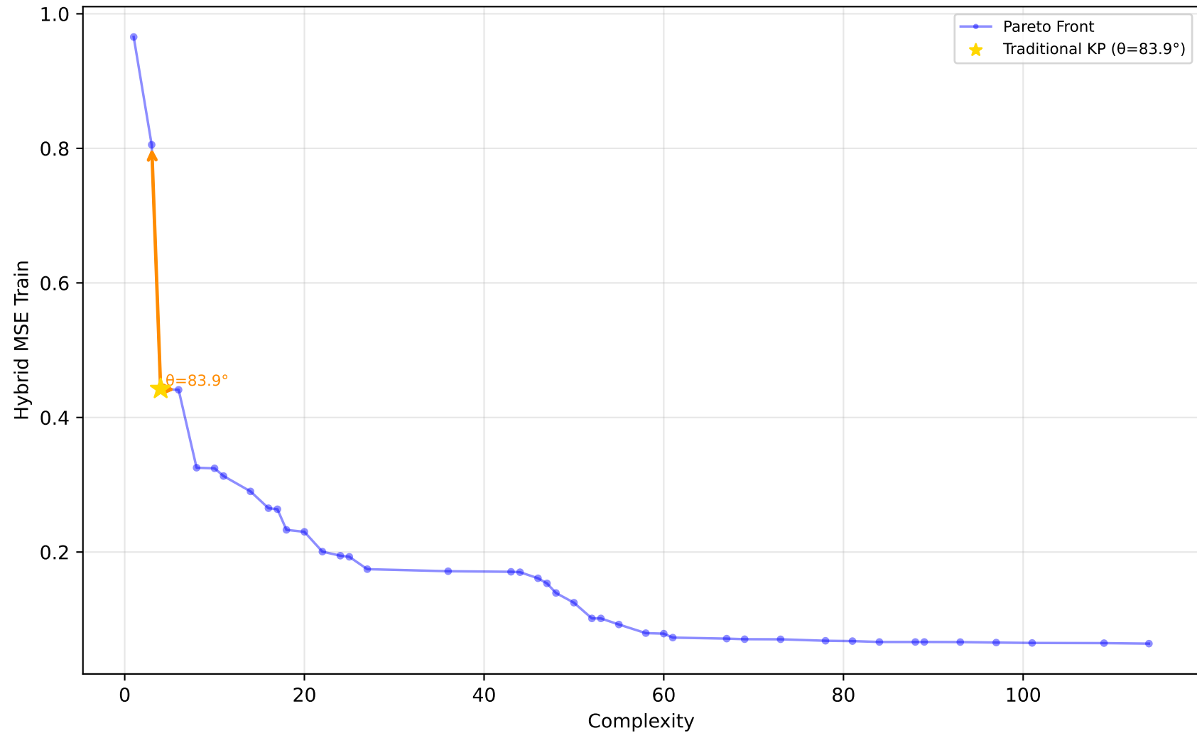
589_fri_c2_1000_25 - Run 22 - SVP - Hybrid MSE Train \lambda_1=0.10, \bar{\lambda}_2=0.00, \bar{\lambda}_3=0.10 | Difficulty: 1.00 | Method: hmr
