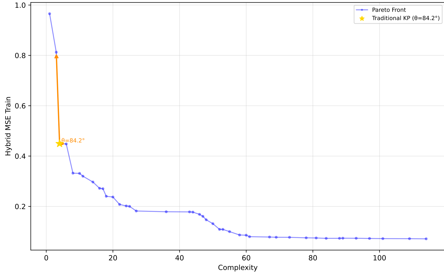
589_fri_c2_1000_25 - Run 22 - SVP - Hybrid MSE Train \lambda_1=0.20, \lambda_2=0.00, \lambda_3=1.00 | Difficulty: 1.00 | Method: hmr
