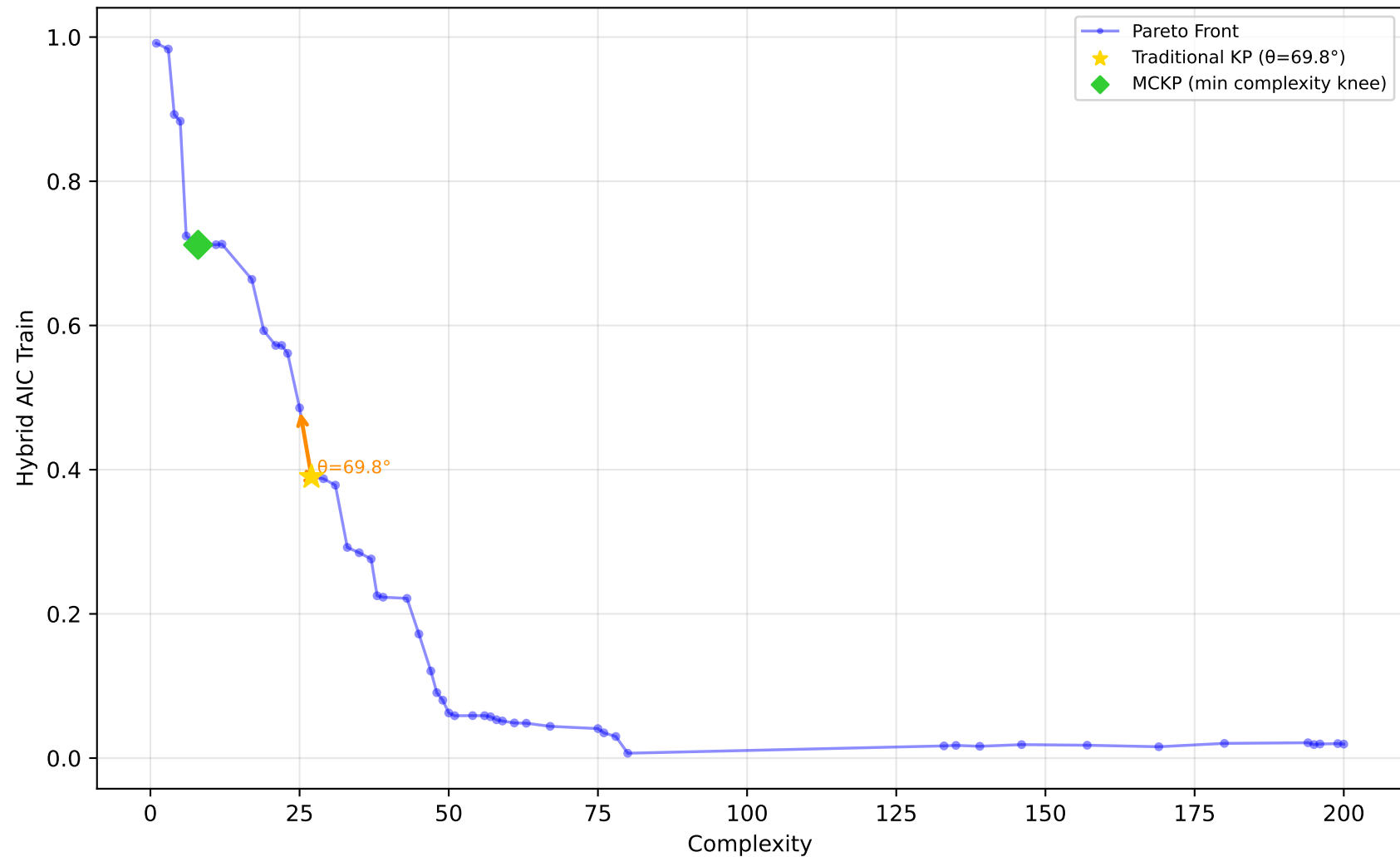
589_fri_c2_1000_25 - Run 23 - SVP - Hybrid AIC Train \lambda_1=0.10, \bar{\lambda}_2=0.00, \bar{\lambda}_3=0.10 | Difficulty: 1.00 | Method: hmr
