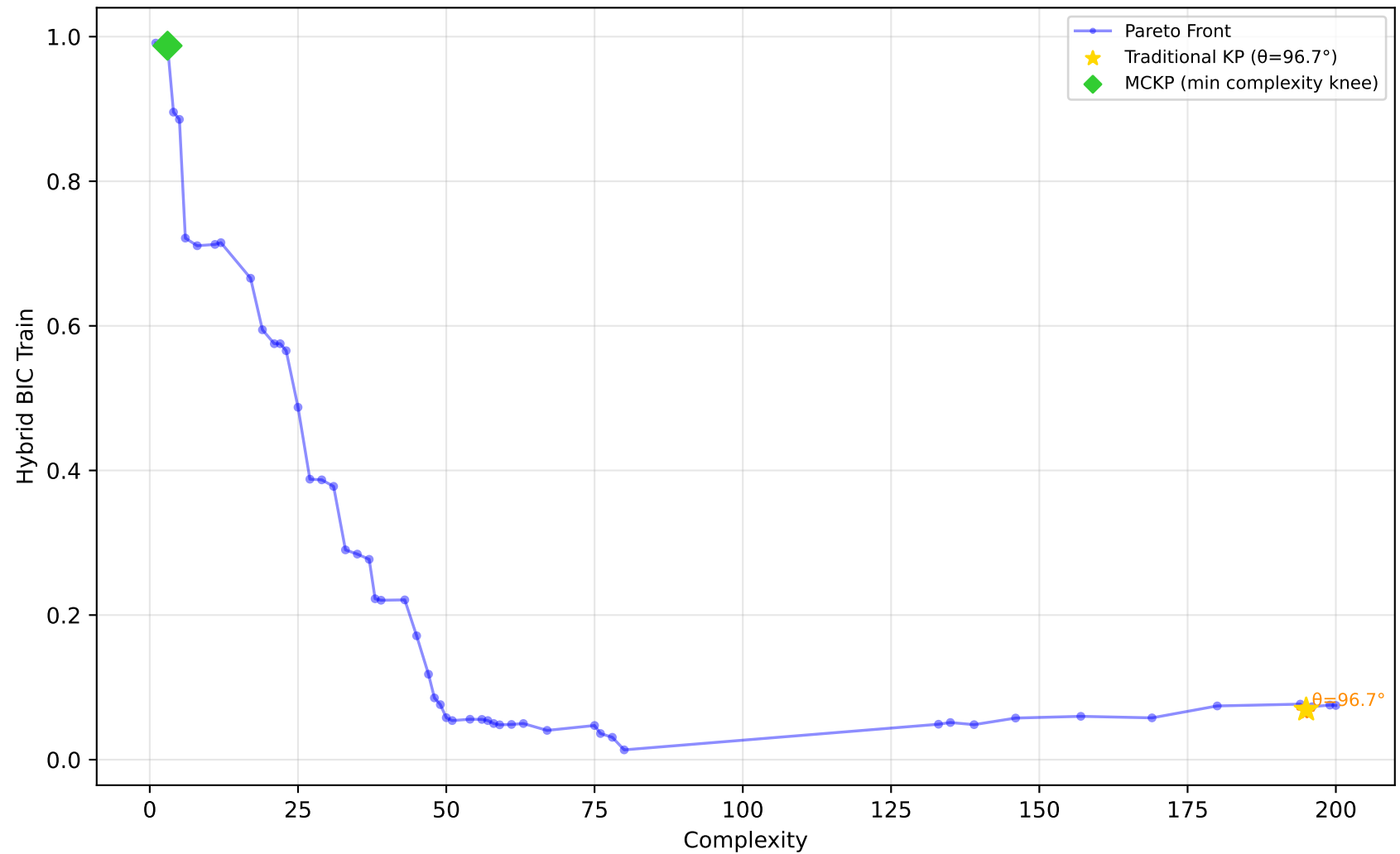
589_fri_c2_1000_25 - Run 23 - SVP - Hybrid BIC Train \lambda_1=0.20, \bar{\lambda}_2=0.00, \bar{\lambda}_3=1.00 | Difficulty: 1.00 | Method: hmr
