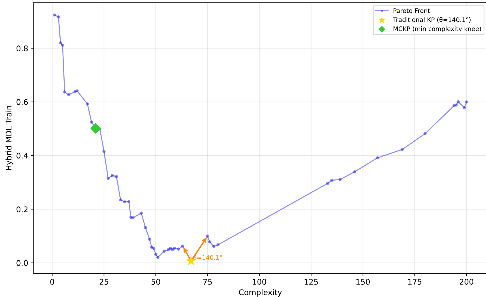
589_fri_c2_1000_25 - Run 23 - SVP - Hybrid MDL Train \lambda_1=0.10, \bar{\lambda}_2=0.00, \bar{\lambda}_3=0.10 | Difficulty: 1.00 | Method: hmr
