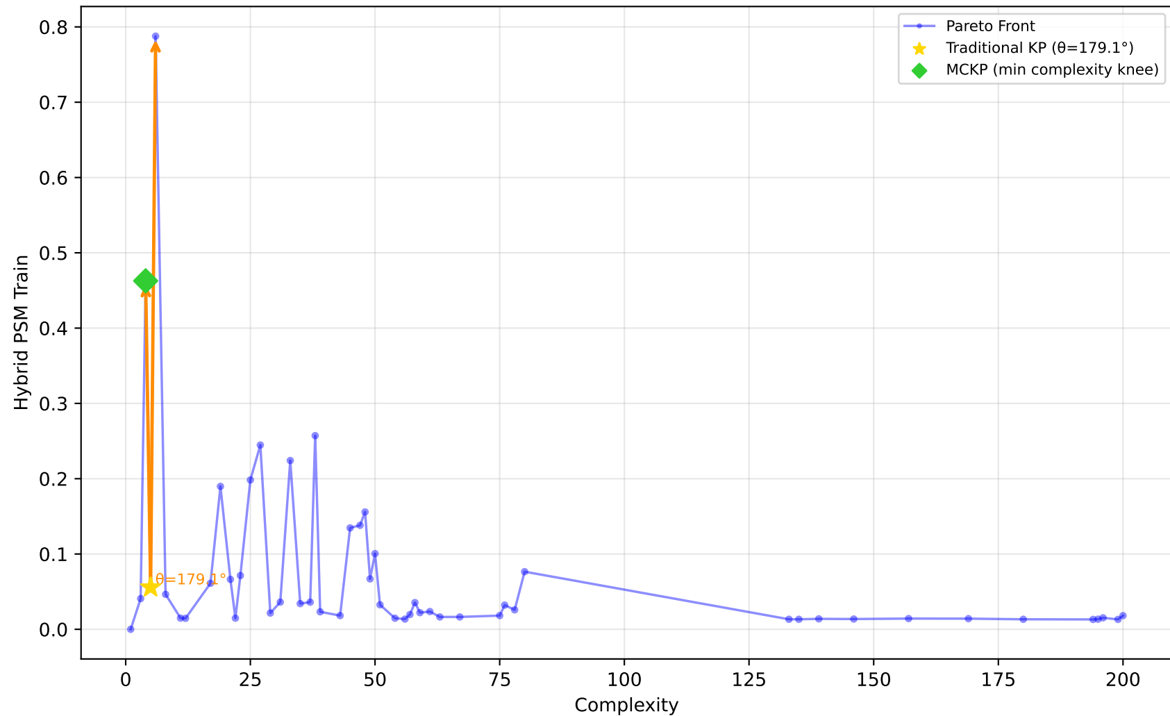
589_fri_c2_1000_25 - Run 23 - SVP - Hybrid PSM Train \lambda_1=0.20, \bar{\lambda}_2=0.00, \bar{\lambda}_3=1.00 | Difficulty: 1.00 | Method: hmr
