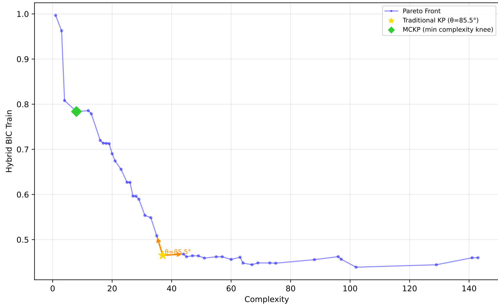
589_fri_c2_1000_25 - Run 24 - MVP - Hybrid BIC Train \lambda_1=0.30, \bar{\lambda}_2=0.00, \bar{\lambda}_3=0.20 | Difficulty: 1.00 | Method: hmr
