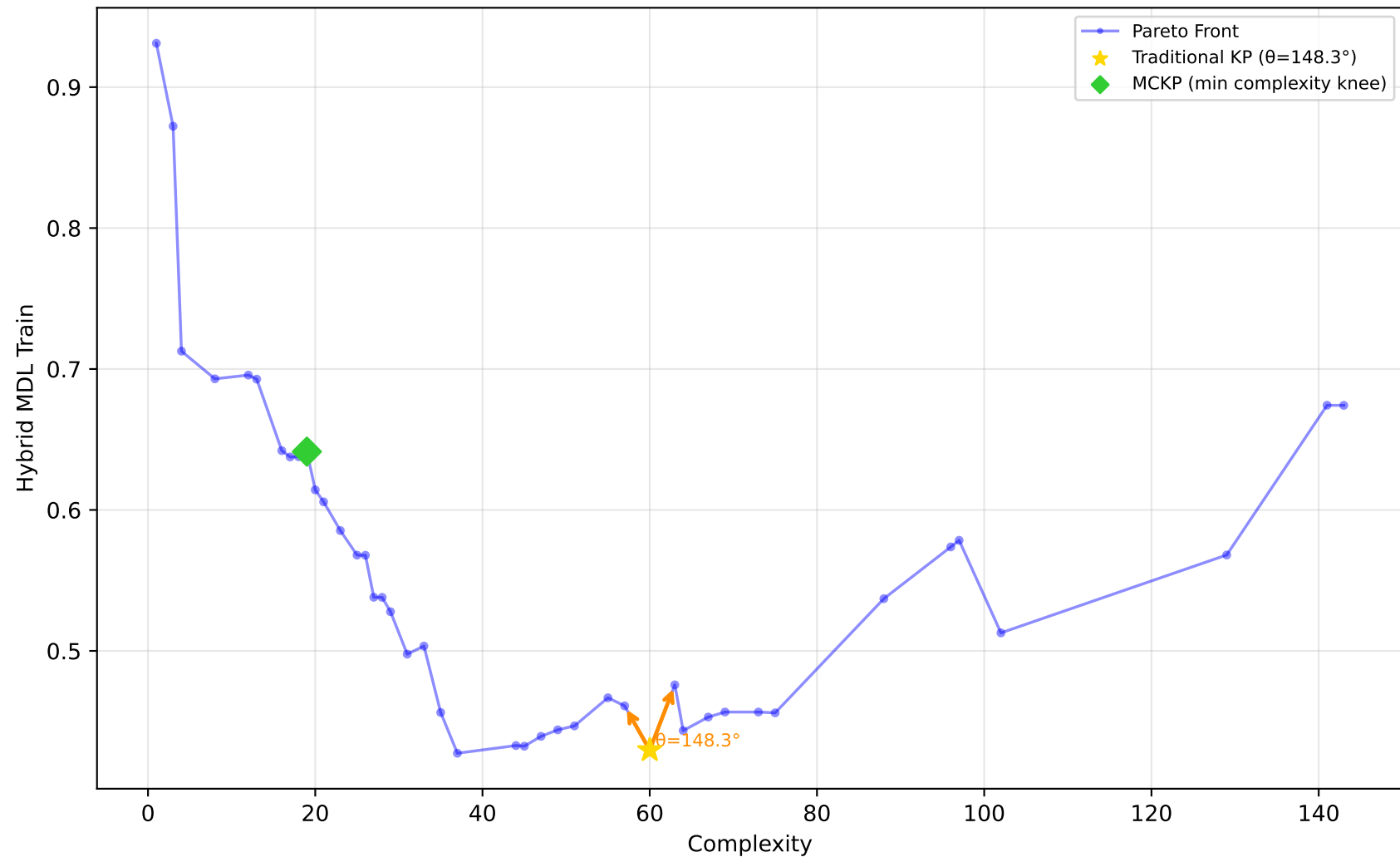
589_fri_c2_1000_25 - Run 24 - MVP - Hybrid MDL Train \lambda_1=0.00, \bar{\lambda}_2=0.00, \bar{\lambda}_3=0.00 | Difficulty: 1.00 | Method: hmr
