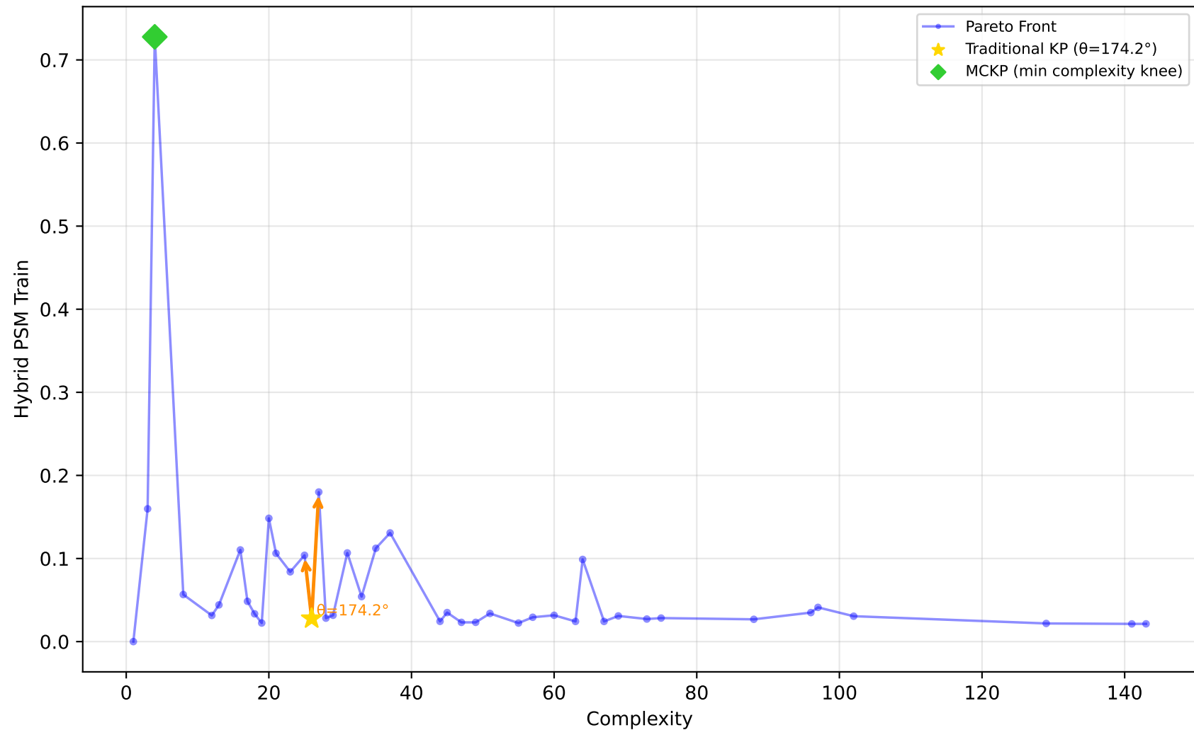
589_fri_c2_1000_25 - Run 24 - MVP - Hybrid PSM Train \lambda_1=0.30, \lambda_2=0.00, \lambda_3=0.20 | Difficulty: 1.00 | Method: hmr
