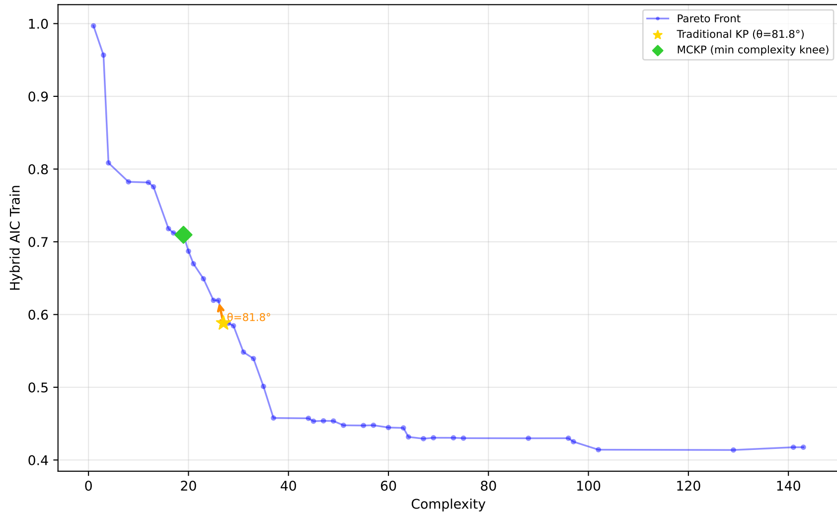
589_fri_c2_1000_25 - Run 24 - SVP - Hybrid AIC Train \lambda_1=0.20, \bar{\lambda}_2=0.00, \bar{\lambda}_3=1.00 | Difficulty: 1.00 | Method: hmr
