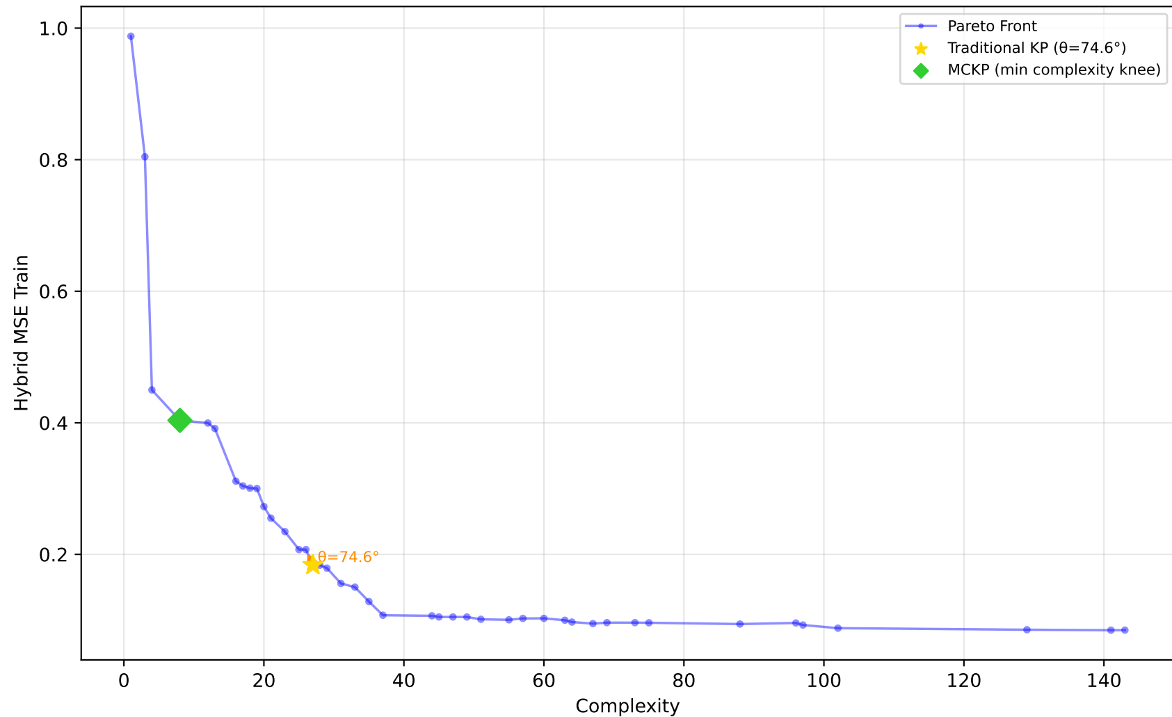
589_fri_c2_1000_25 - Run 24 - SVP - Hybrid MSE Train \lambda_1=0.20, \bar{\lambda}_2=0.00, \bar{\lambda}_3=1.00 | Difficulty: 1.00 | Method: hmr
