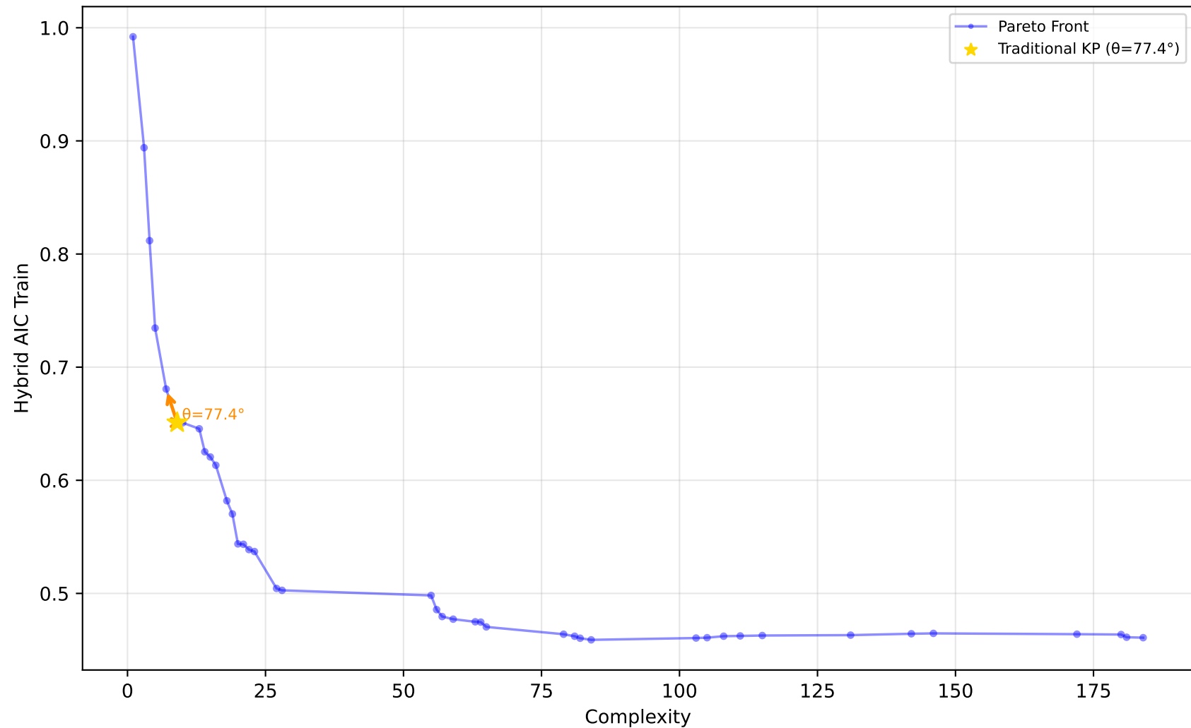
589_fri_c2_1000_25 - Run 25 - MVP - Hybrid AIC Train \lambda_1=0.00, \lambda_2=0.00, \lambda_3=0.00 | Difficulty: 1.00 | Method: hmr
