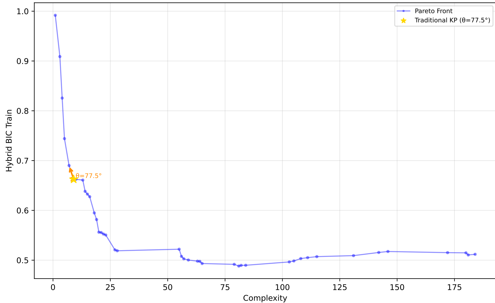
589_fri_c2_1000_25 - Run 25 - MVP - Hybrid BIC Train \lambda_1=0.30, \bar{\lambda}_2=0.00, \bar{\lambda}_3=0.20 | Difficulty: 1.00 | Method: hmr
