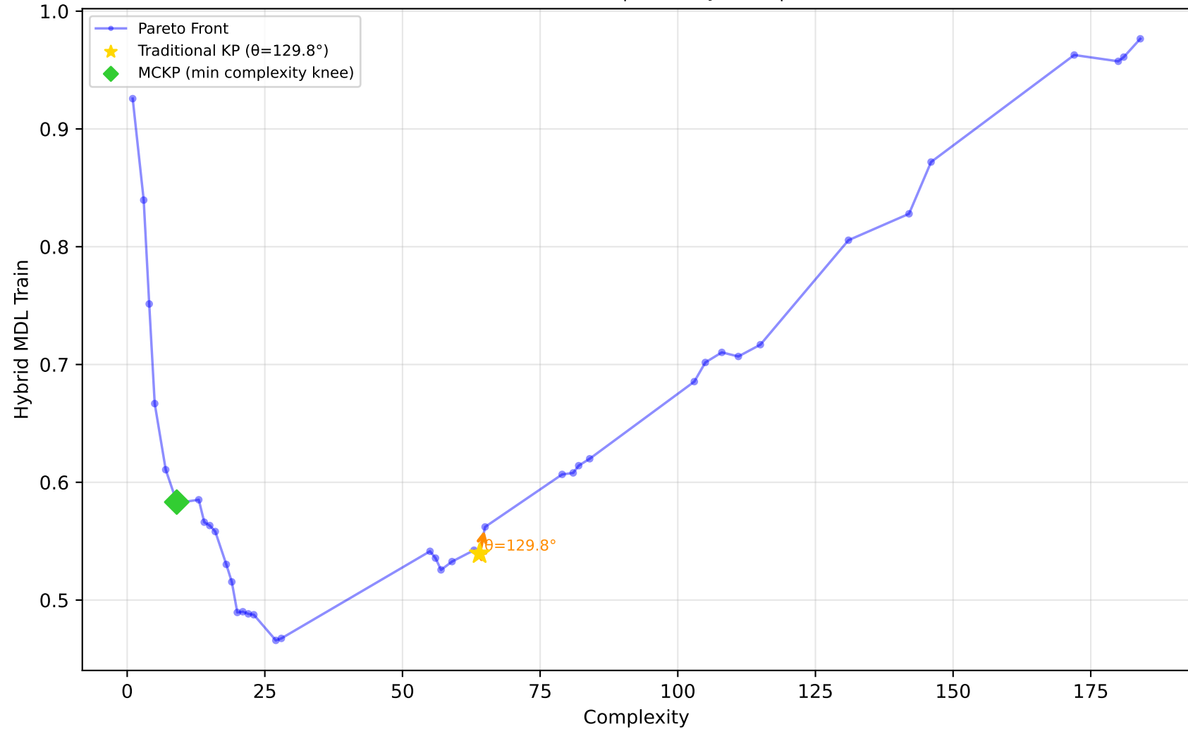
589_fri_c2_1000_25 - Run 25 - MVP - Hybrid MDL Train \lambda_1=0.30, \lambda_2=0.00, \lambda_3=0.20 | Difficulty: 1.00 | Method: hmr
