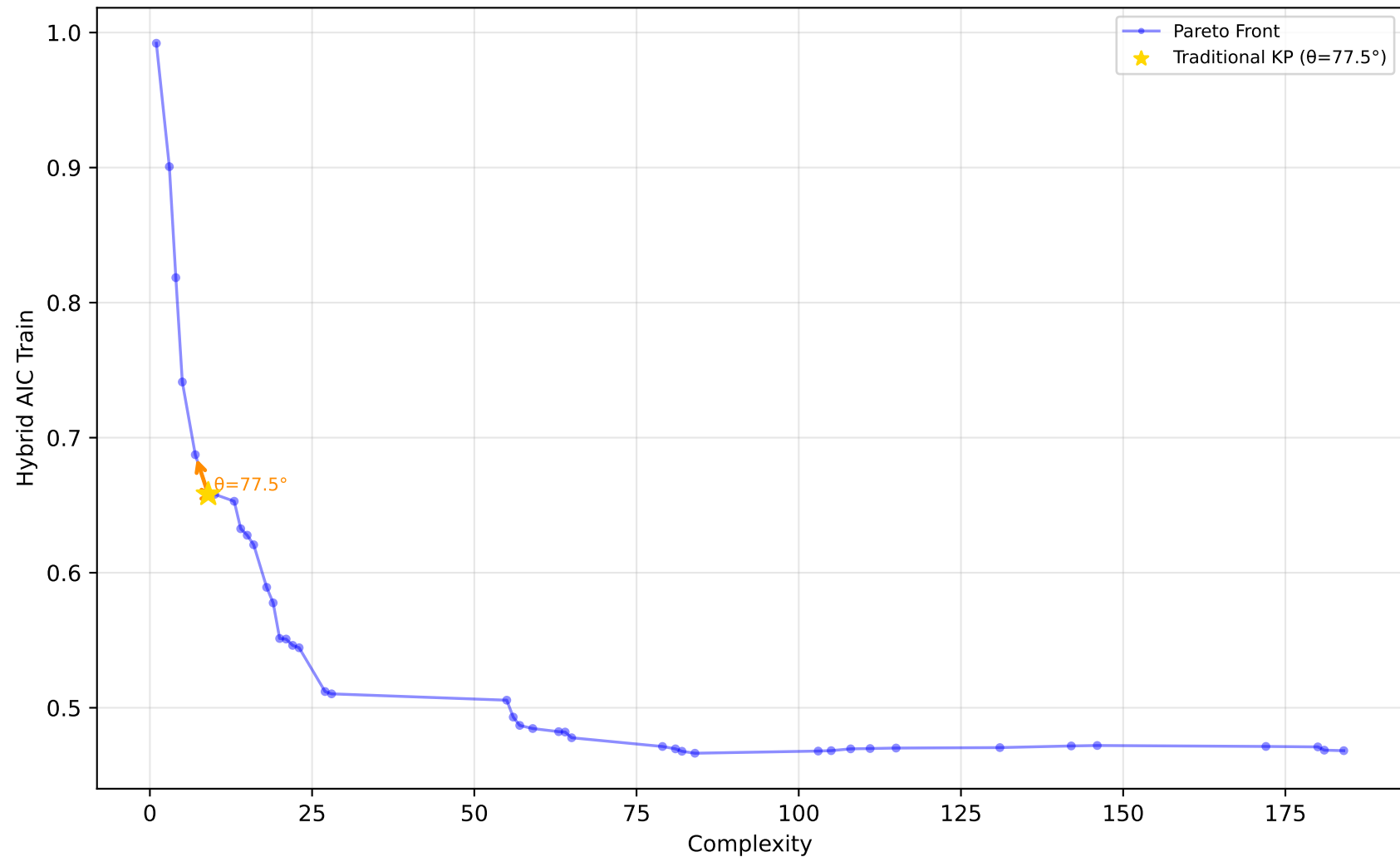
589_fri_c2_1000_25 - Run 25 - SVP - Hybrid AIC Train \lambda_1=0.10, \bar{\lambda}_2=0.00, \bar{\lambda}_3=0.10 | Difficulty: 1.00 | Method: hmr
