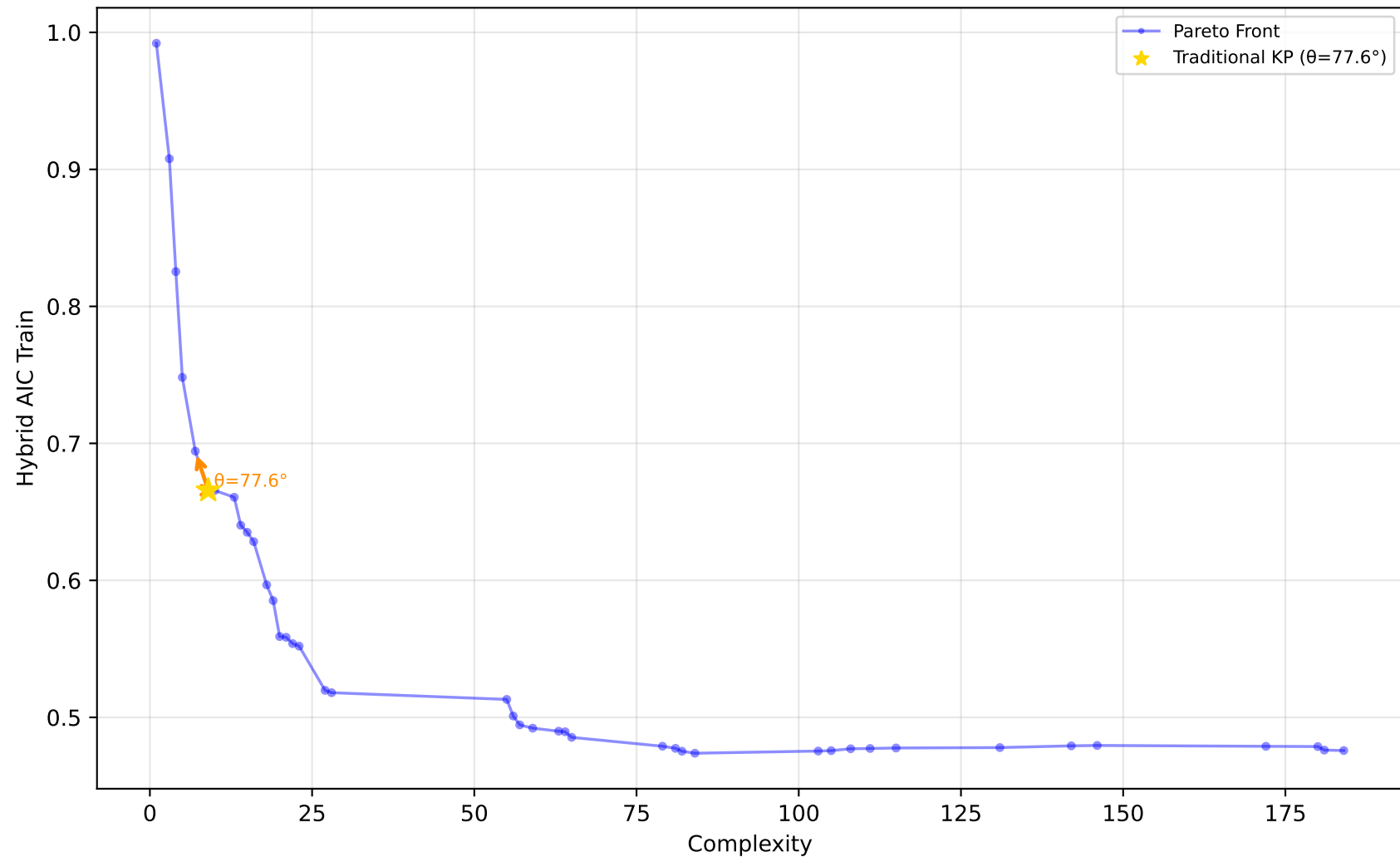
589_fri_c2_1000_25 - Run 25 - SVP - Hybrid AIC Train \lambda_1=0.20, \bar{\lambda}_2=0.00, \bar{\lambda}_3=1.00 | Difficulty: 1.00 | Method: hmr
