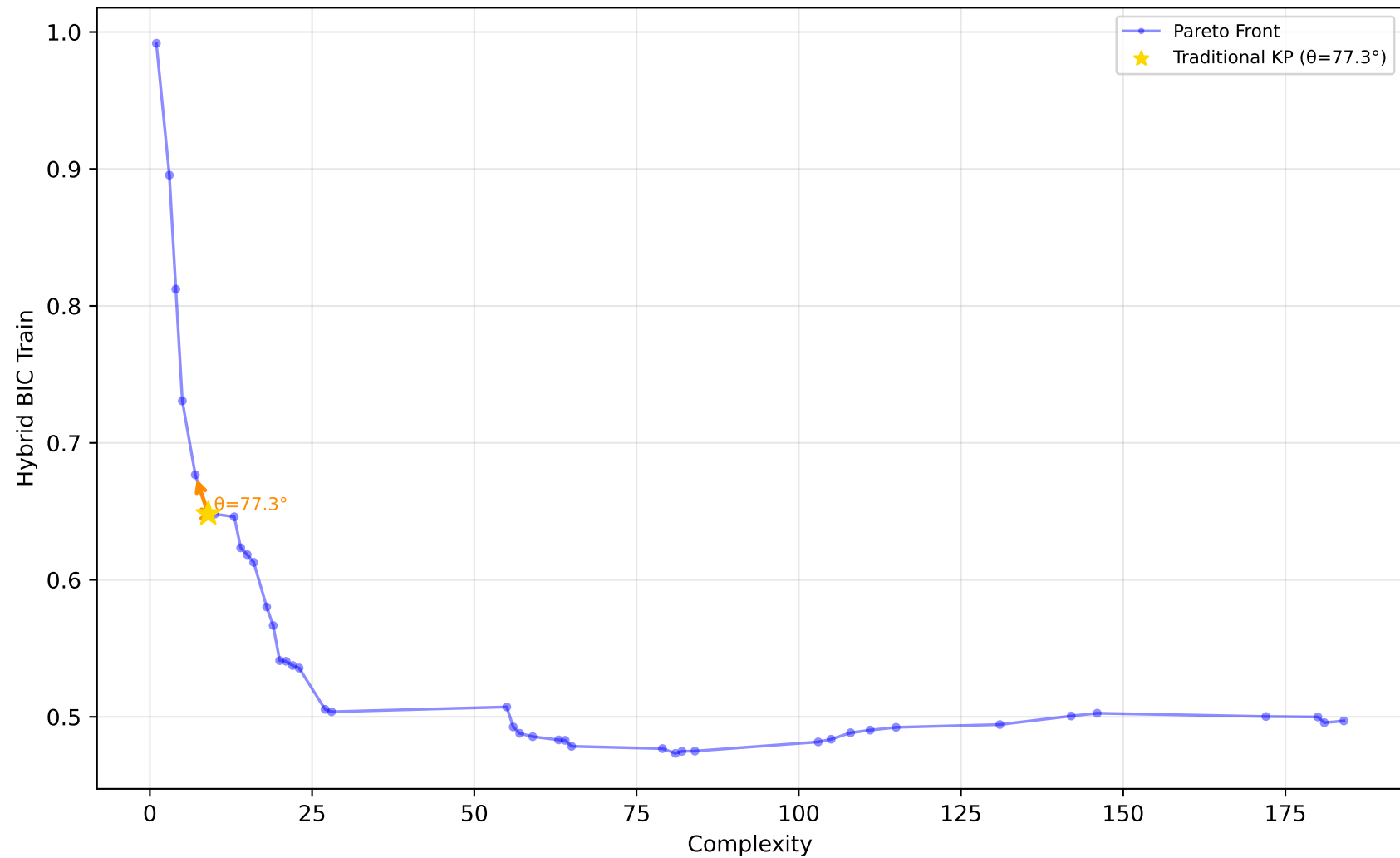
589_fri_c2_1000_25 - Run 25 - SVP - Hybrid BIC Train \lambda_1=0.10, \bar{\lambda}_2=0.00, \bar{\lambda}_3=0.10 | Difficulty: 1.00 | Method: hmr
