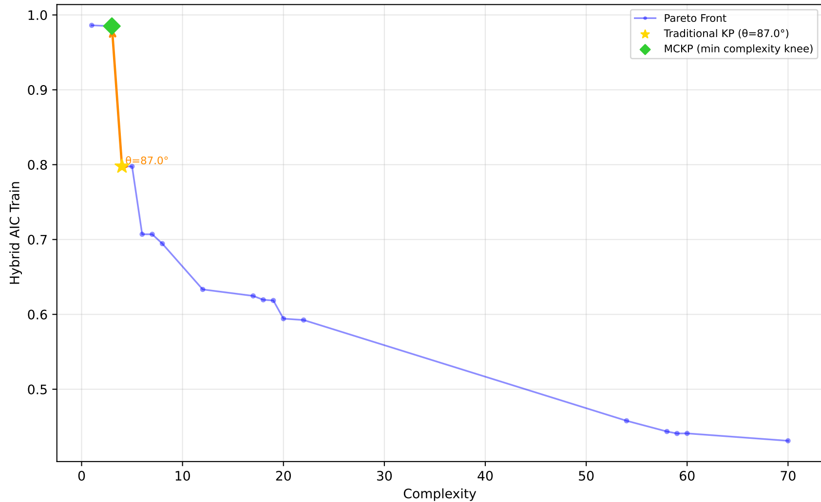
589_fri_c2_1000_25 - Run 26 - MVP - Hybrid AIC Train \lambda_1=0.00, \bar{\lambda}_2=0.00, \bar{\lambda}_3=0.00 | Difficulty: 1.00 | Method: hmr
