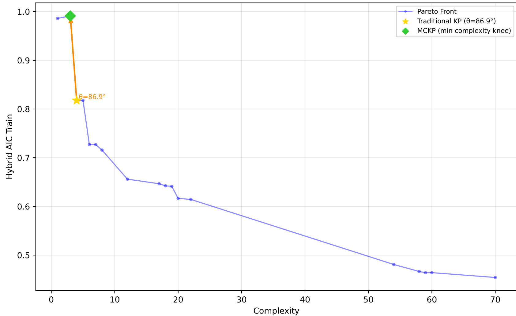
589_fri_c2_1000_25 - Run 26 - MVP - Hybrid AIC Train \lambda_1=0.30, \bar{\lambda}_2=0.00, \bar{\lambda}_3=0.20 | Difficulty: 1.00 | Method: hmr
