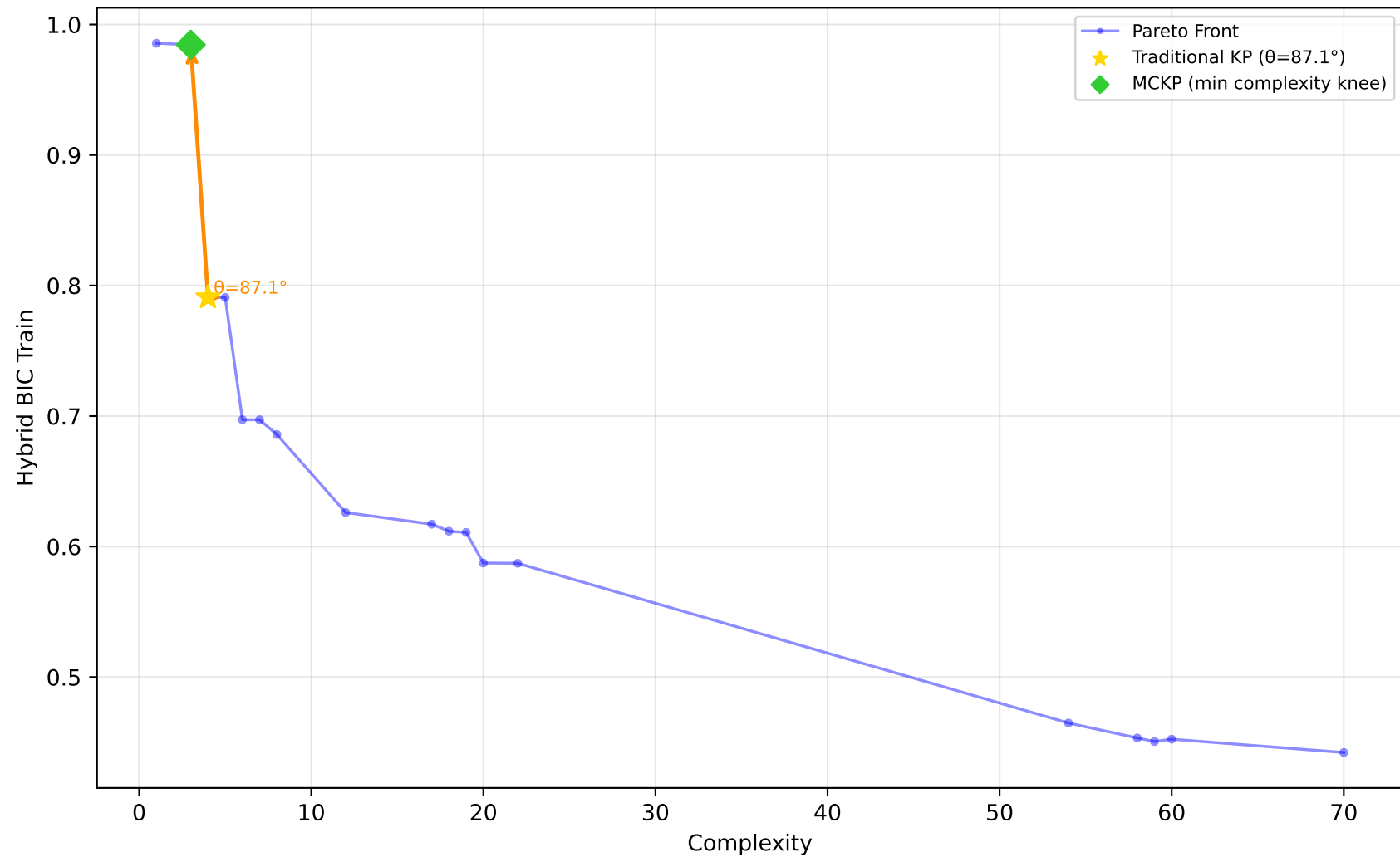
589_fri_c2_1000_25 - Run 26 - MVP - Hybrid BIC Train \lambda_1=0.00, \bar{\lambda}_2=0.00, \bar{\lambda}_3=0.00 | Difficulty: 1.00 | Method: hmr
