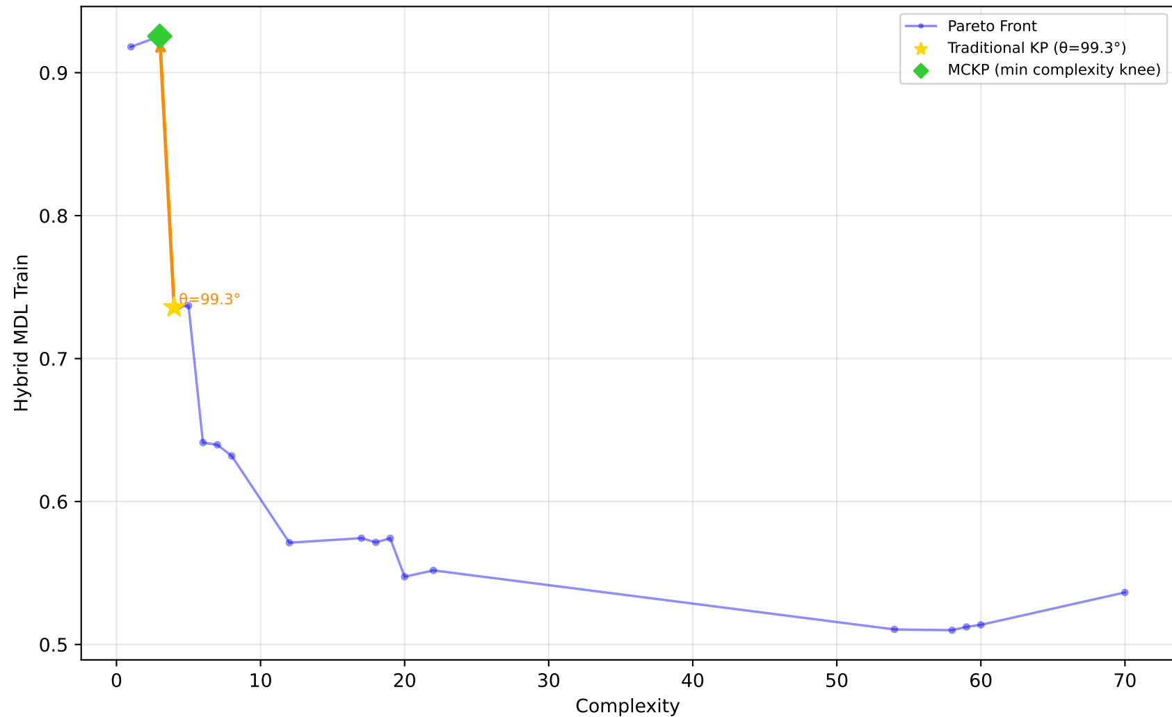
589_fri_c2_1000_25 - Run 26 - MVP - Hybrid MDL Train \lambda_1=0.30, \lambda_2=0.00, \lambda_3=0.20 | Difficulty: 1.00 | Method: hmr
