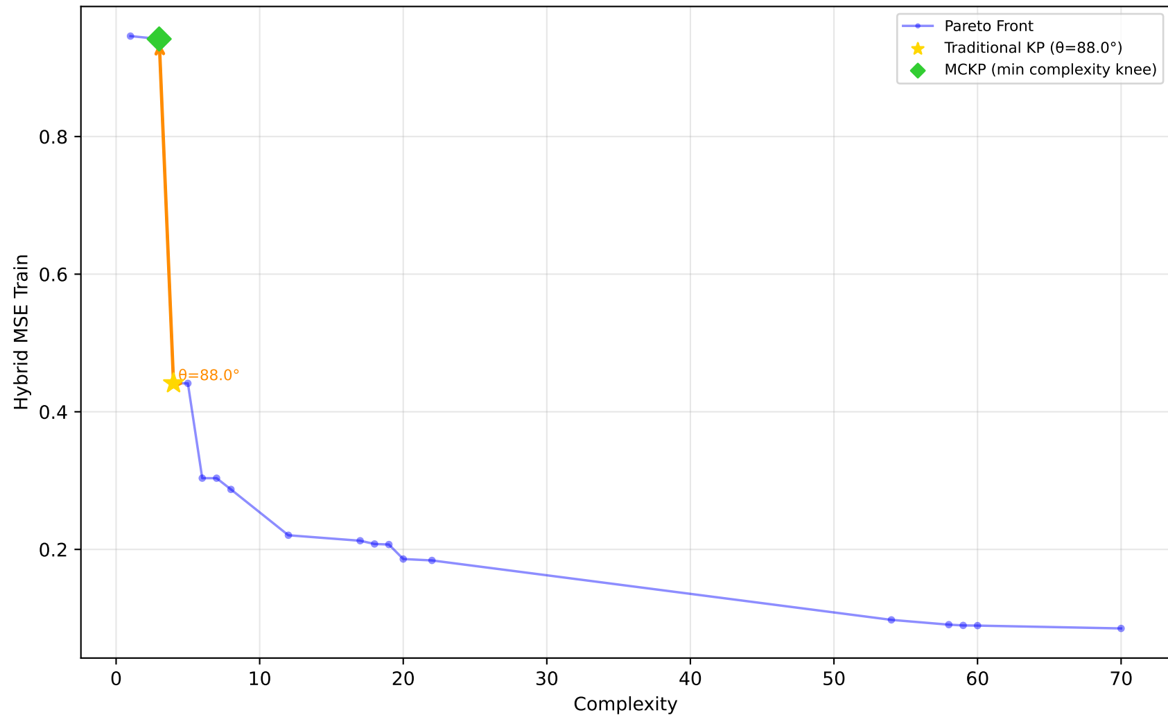
589_fri_c2_1000_25 - Run 26 - MVP - Hybrid MSE Train \lambda_1=0.00, \bar{\lambda}_2=0.00, \bar{\lambda}_3=0.00 | Difficulty: 1.00 | Method: hmr
