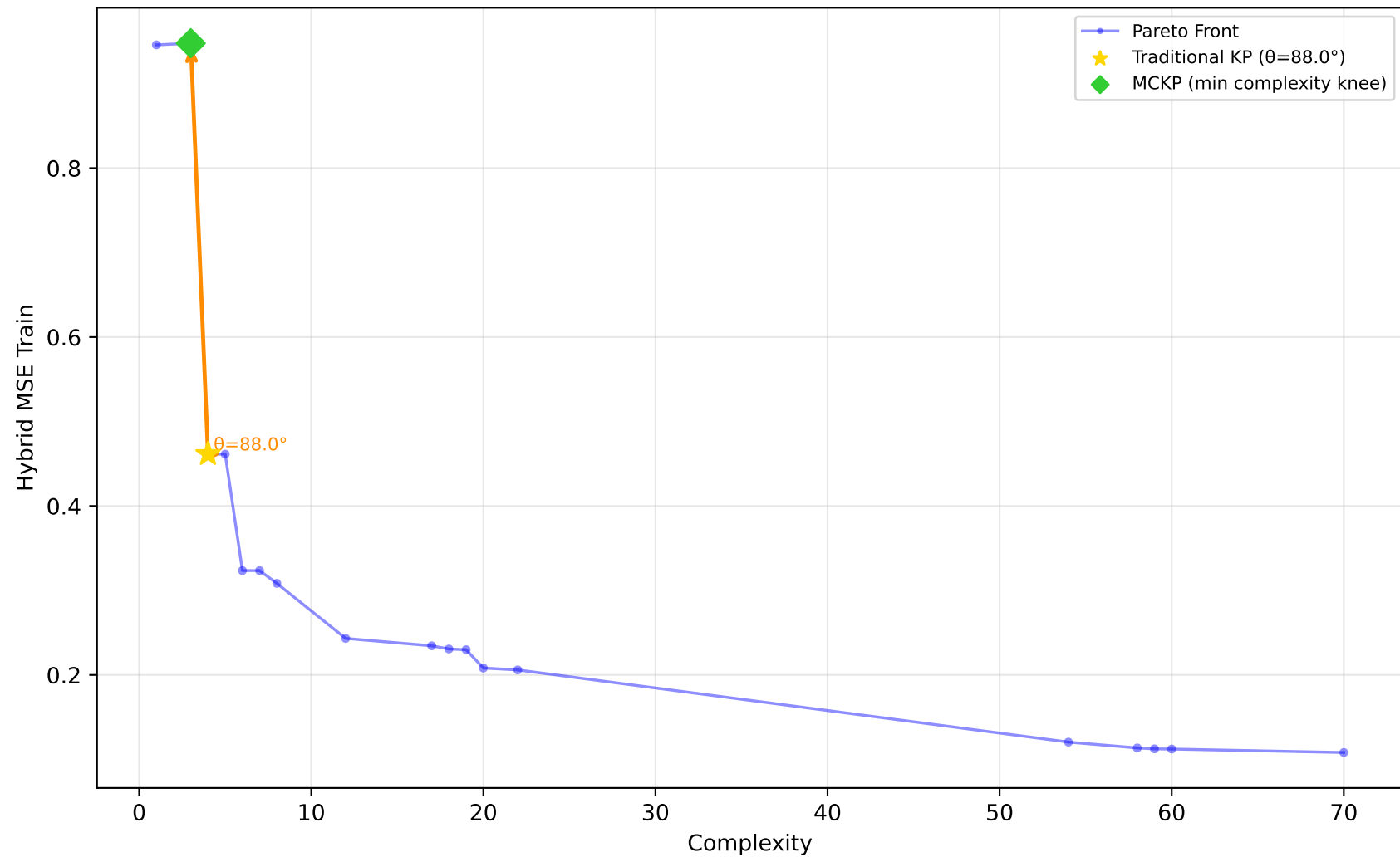
589_fri_c2_1000_25 - Run 26 - MVP - Hybrid MSE Train \lambda_1=0.30, \lambda_2=0.00, \lambda_3=0.20 | Difficulty: 1.00 | Method: hmr
