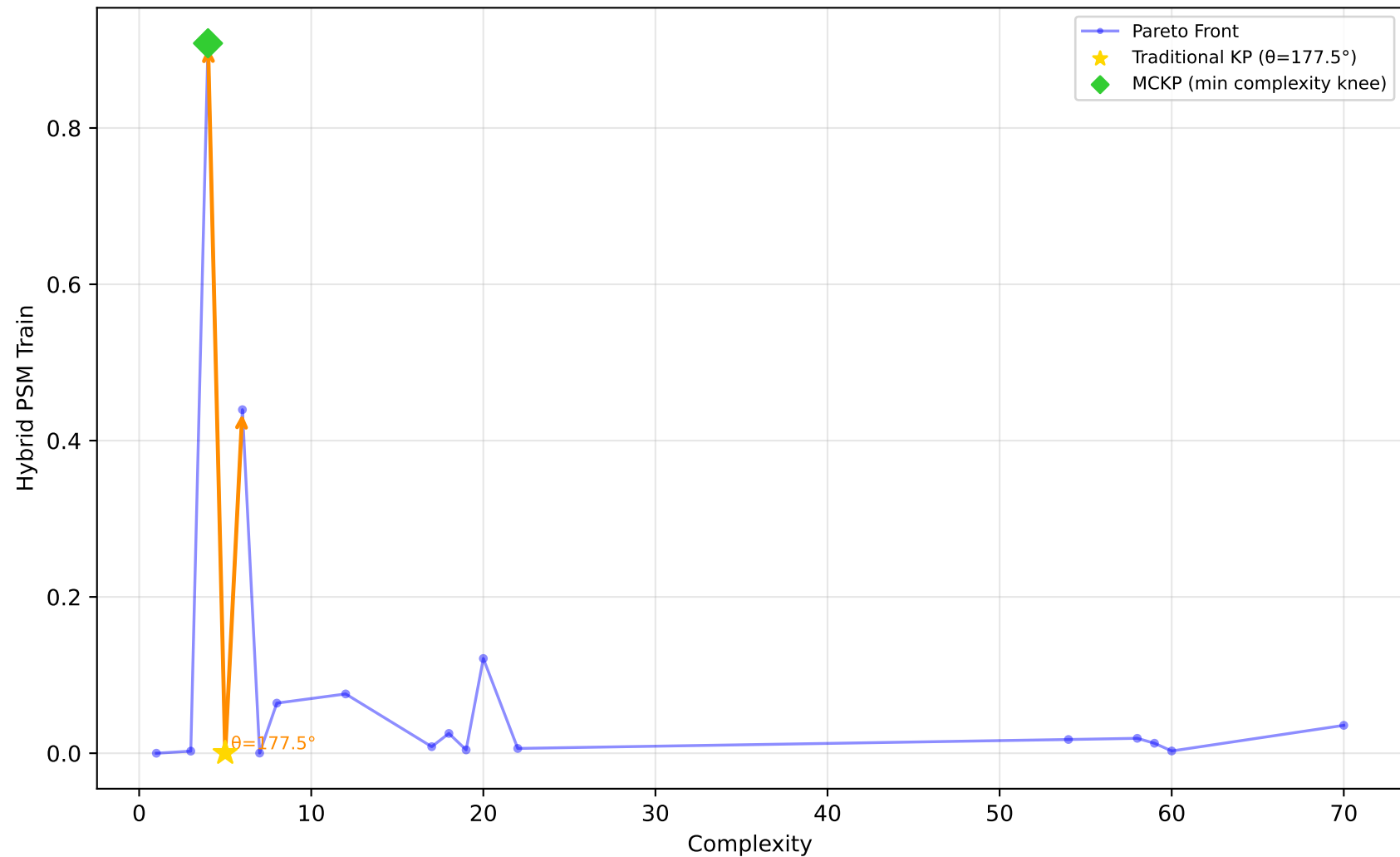
589_fri_c2_1000_25 - Run 26 - MVP - Hybrid PSM Train \lambda_1=0.00, \lambda_2=0.00, \lambda_3=0.00 | Difficulty: 1.00 | Method: hmr
