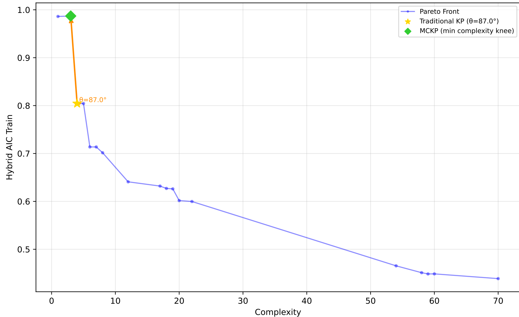
589_fri_c2_1000_25 - Run 26 - SVP - Hybrid AIC Train \lambda_1=0.10, \bar{\lambda}_2=0.00, \bar{\lambda}_3=0.10 | Difficulty: 1.00 | Method: hmr
