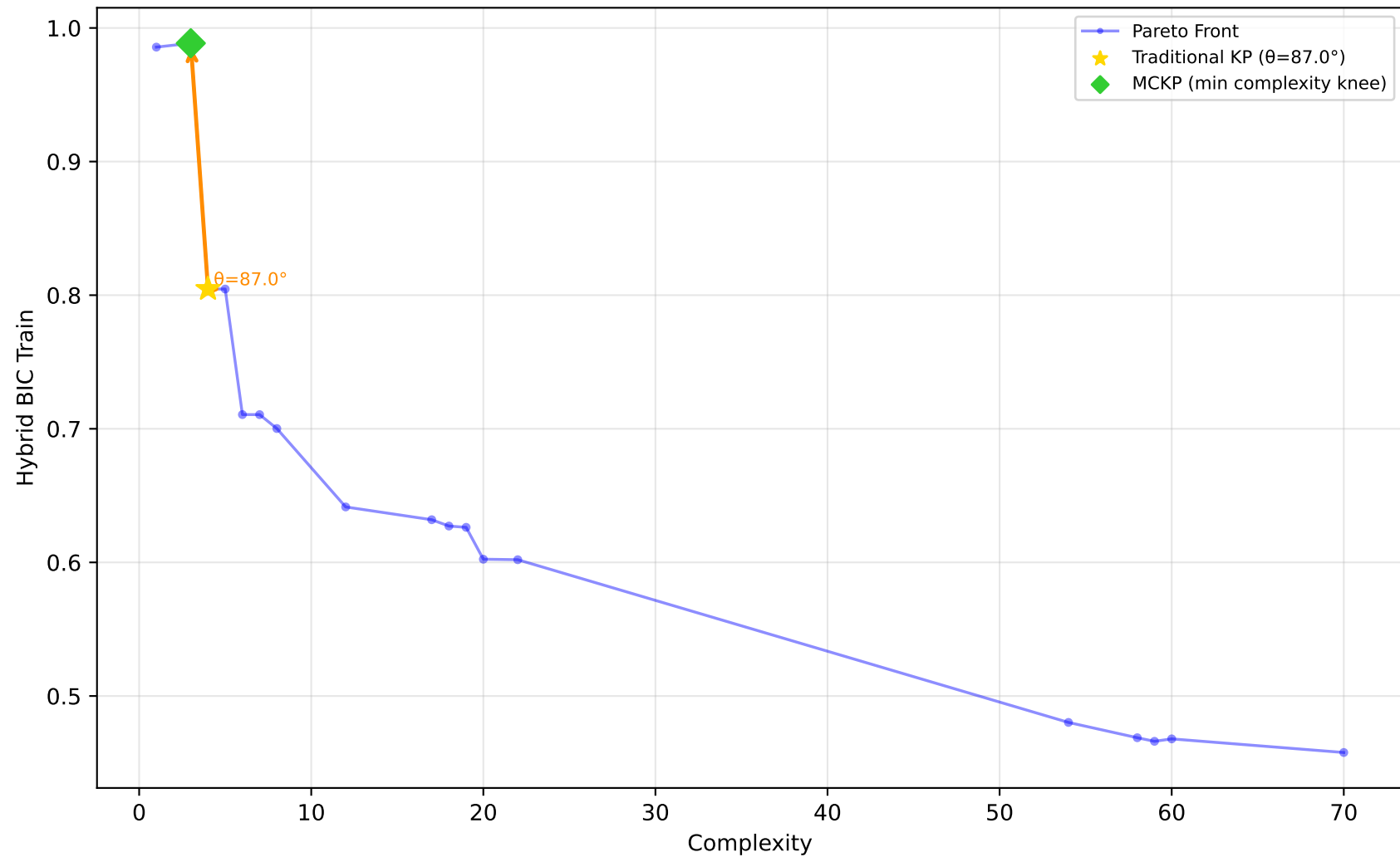
589_fri_c2_1000_25 - Run 26 - SVP - Hybrid BIC Train \lambda_1=0.20, \bar{\lambda}_2=0.00, \bar{\lambda}_3=1.00 | Difficulty: 1.00 | Method: hmr
