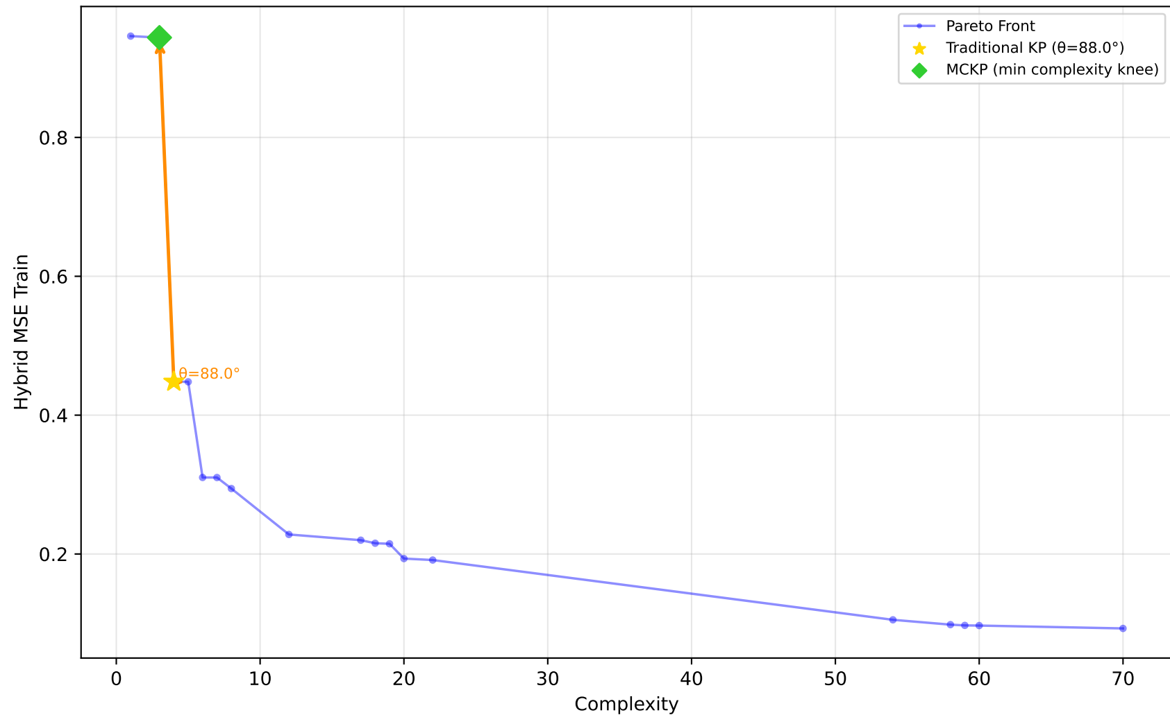
589_fri_c2_1000_25 - Run 26 - SVP - Hybrid MSE Train \lambda_1=0.10, \bar{\lambda}_2=0.00, \bar{\lambda}_3=0.10 | Difficulty: 1.00 | Method: hmr
