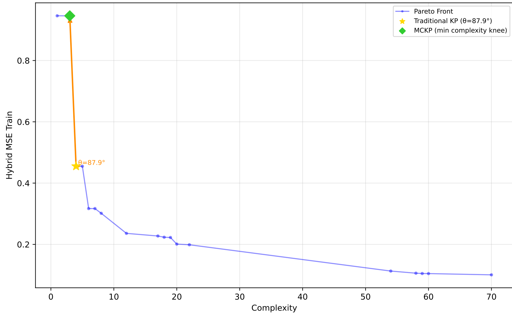
589_fri_c2_1000_25 - Run 26 - SVP - Hybrid MSE Train \lambda_1=0.20, \lambda_2=0.00, \lambda_3=1.00 | Difficulty: 1.00 | Method: hmr
