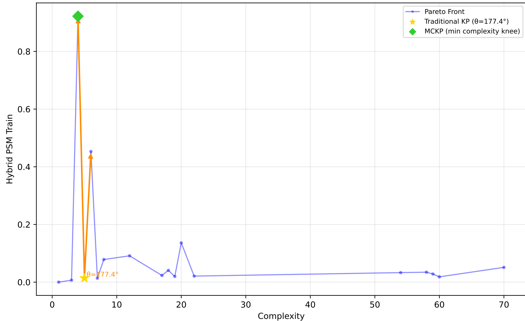
589_fri_c2_1000_25 - Run 26 - SVP - Hybrid PSM Train \lambda_1=0.20, \lambda_2=0.00, \lambda_3=1.00 | Difficulty: 1.00 | Method: hmr
