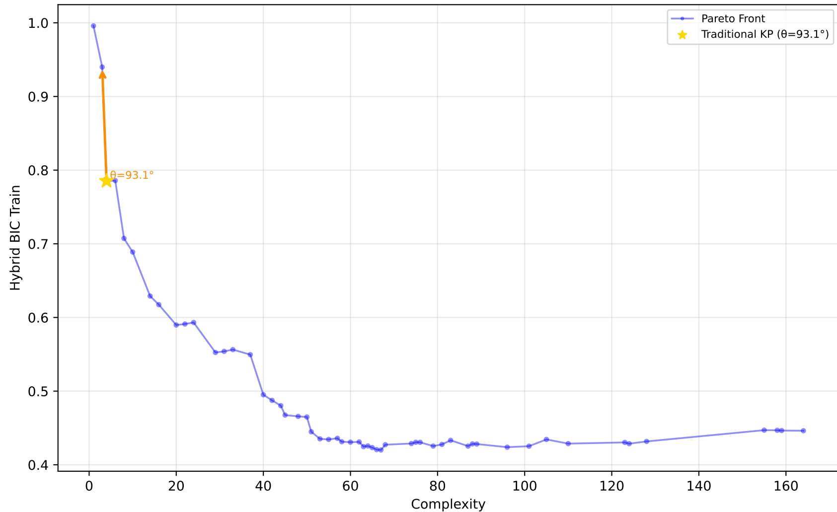
589_fri_c2_1000_25 - Run 27 - MVP - Hybrid BIC Train \lambda_1=0.00, \bar{\lambda}_2=0.00, \bar{\lambda}_3=0.00 | Difficulty: 1.00 | Method: hmr
