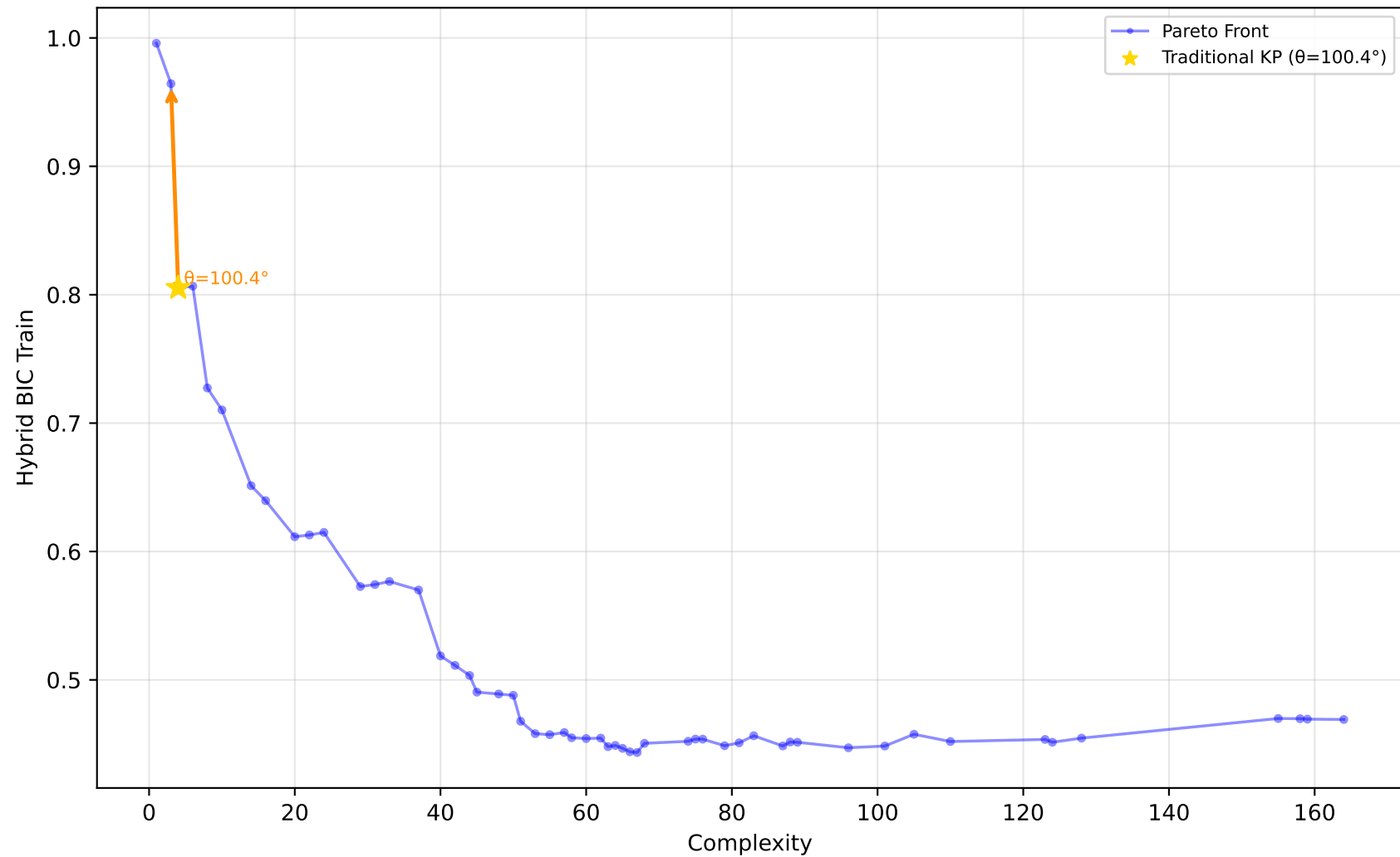
589_fri_c2_1000_25 - Run 27 - MVP - Hybrid BIC Train \lambda_1=0.30, \bar{\lambda}_2=0.00, \bar{\lambda}_3=0.20 | Difficulty: 1.00 | Method: hmr
