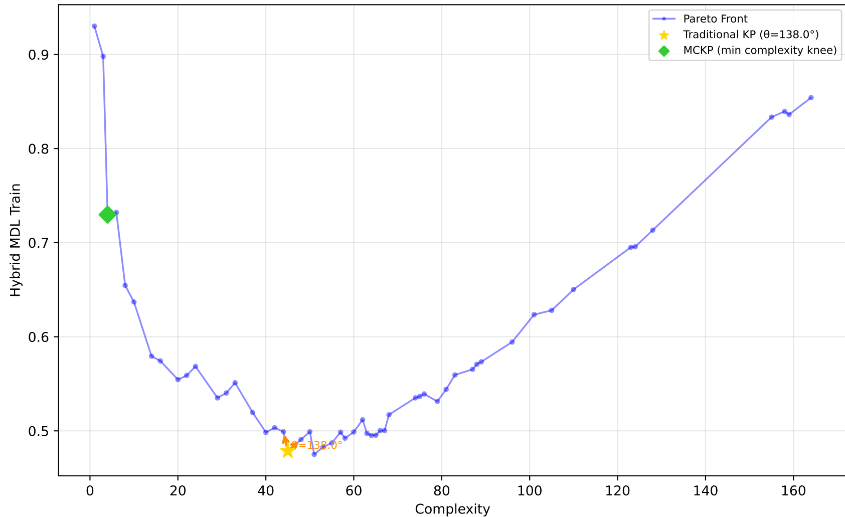
589_fri_c2_1000_25 - Run 27 - MVP - Hybrid MDL Train \lambda_1=0.30, \lambda_2=0.00, \lambda_3=0.20 | Difficulty: 1.00 | Method: hmr
