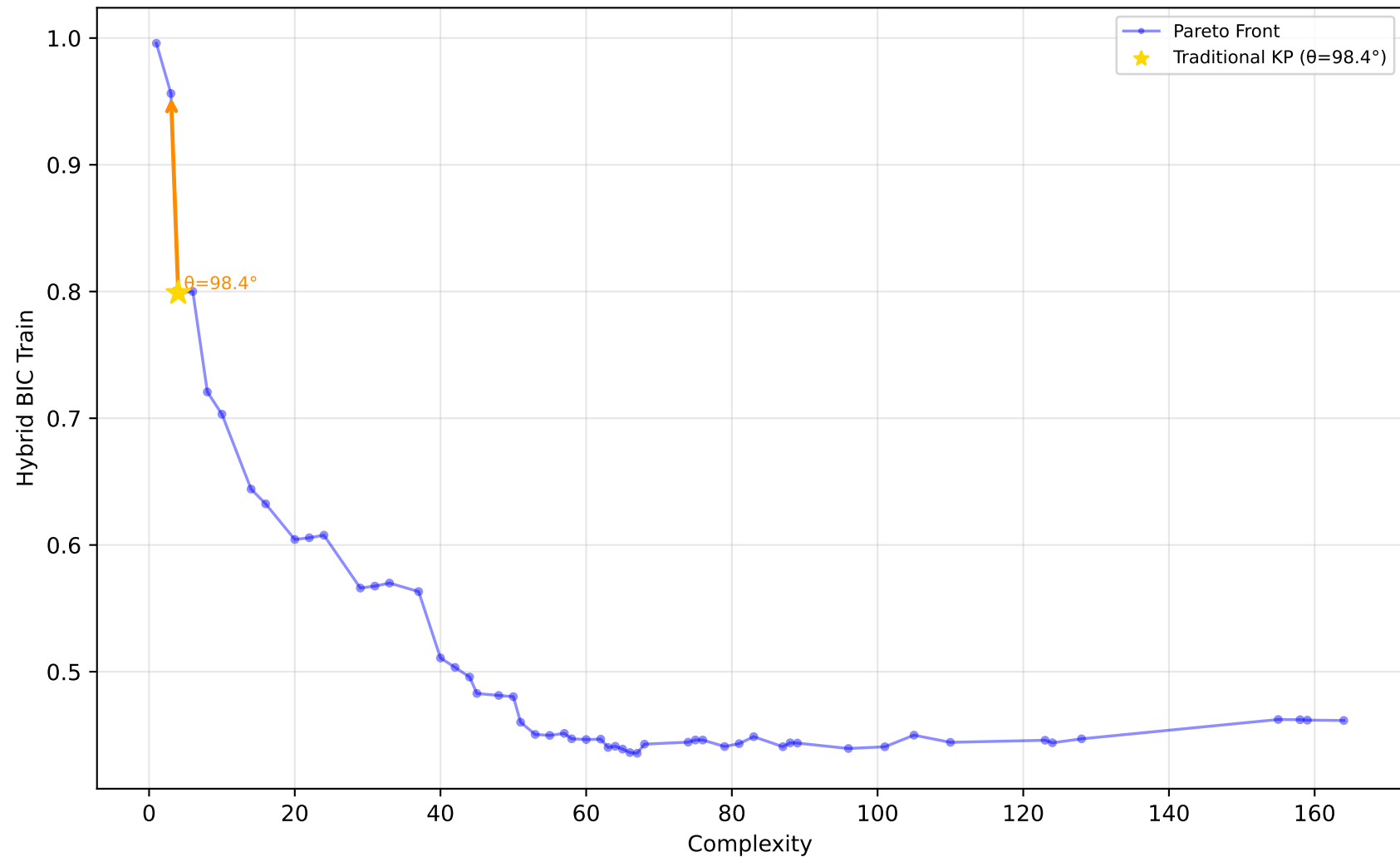
589_fri_c2_1000_25 - Run 27 - SVP - Hybrid BIC Train \lambda_1=0.20, \bar{\lambda}_2=0.00, \bar{\lambda}_3=1.00 | Difficulty: 1.00 | Method: hmr
