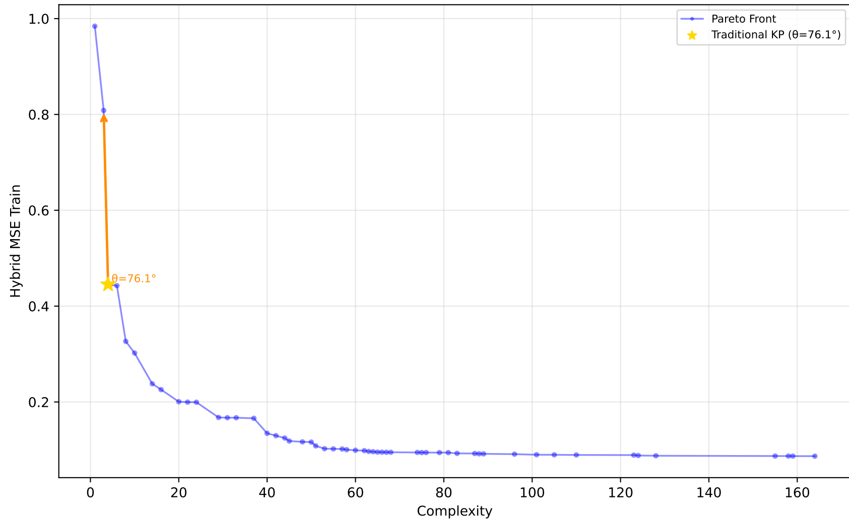
589_fri_c2_1000_25 - Run 27 - SVP - Hybrid MSE Train \lambda_1=0.20, \bar{\lambda}_2=0.00, \bar{\lambda}_3=1.00 | Difficulty: 1.00 | Method: hmr
