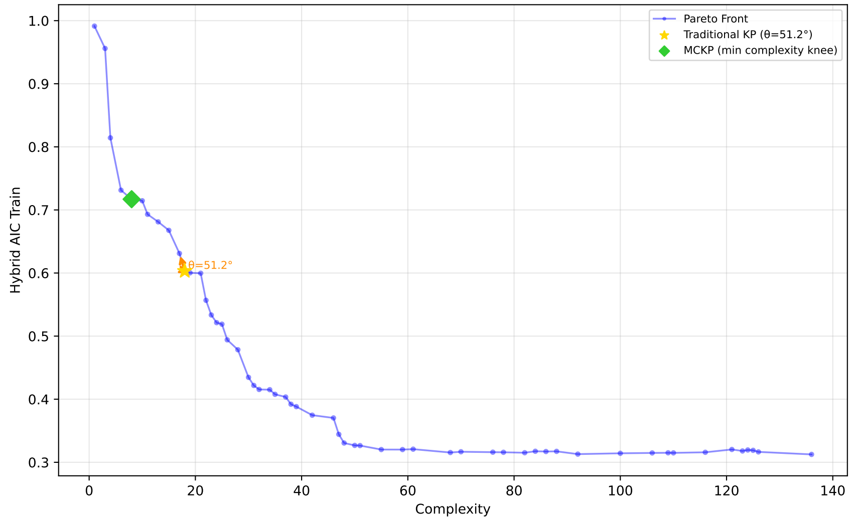
589_fri_c2_1000_25 - Run 28 - MVP - Hybrid AIC Train \lambda_1=0.30, \lambda_2=0.00, \lambda_3=0.20 | Difficulty: 1.00 | Method: hmr
