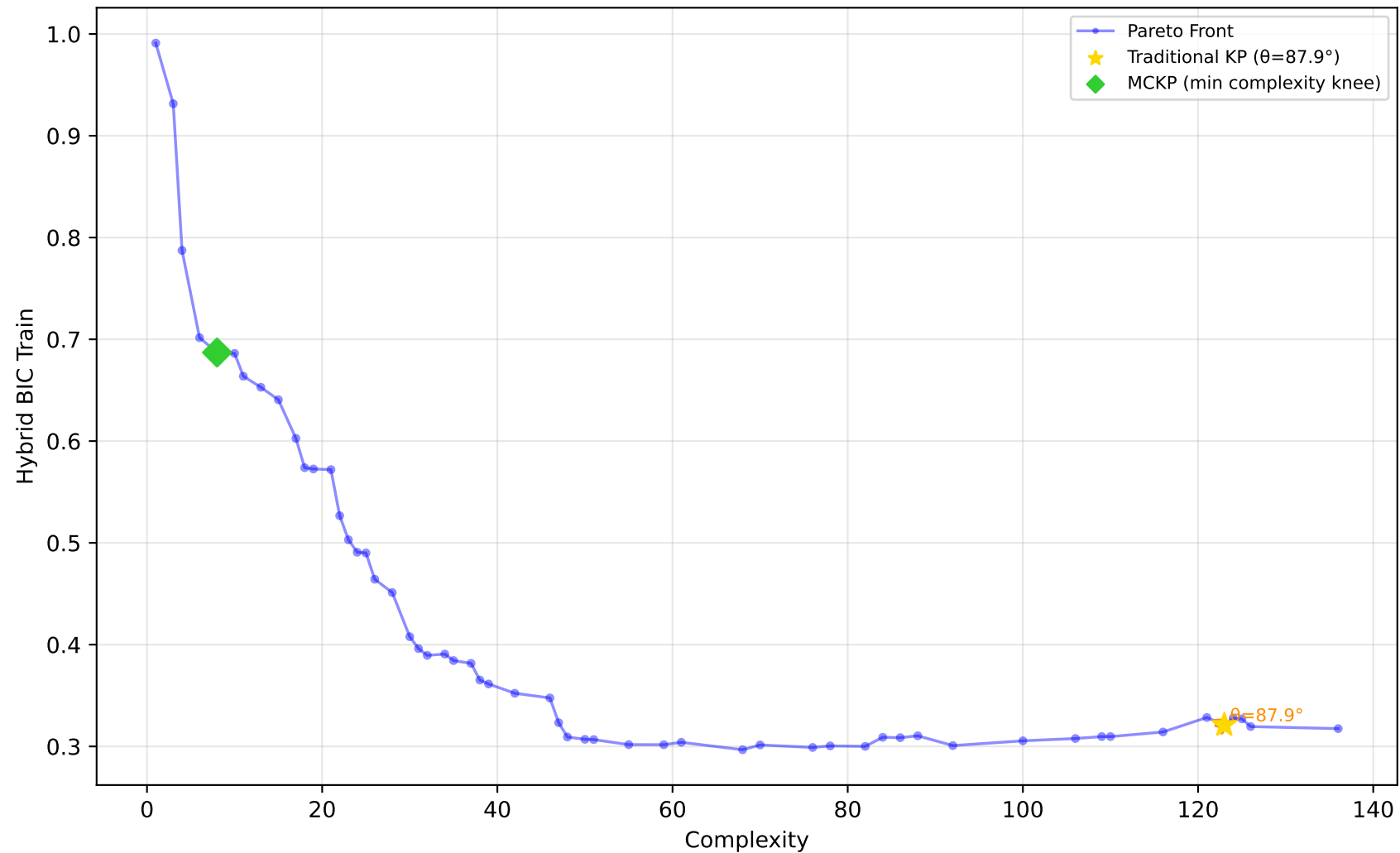
589_fri_c2_1000_25 - Run 28 - MVP - Hybrid BIC Train \lambda_1=0.00, \lambda_2=0.00, \lambda_3=0.00 | Difficulty: 1.00 | Method: hmr
