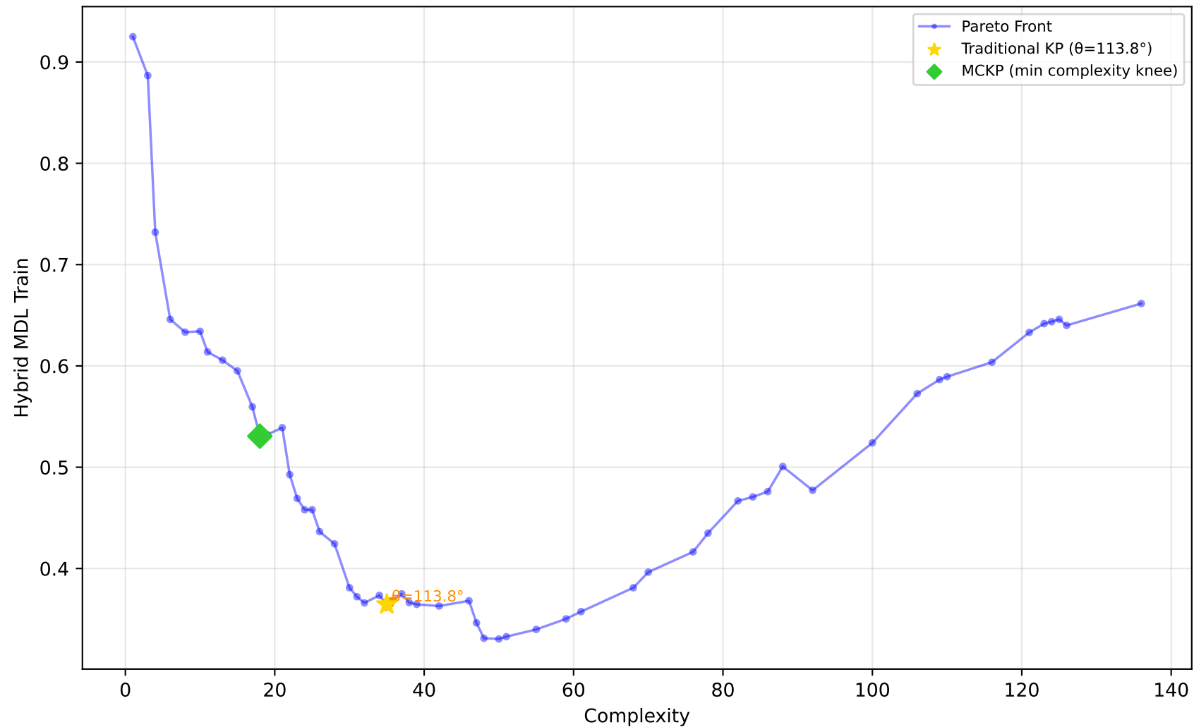
589_fri_c2_1000_25 - Run 28 - MVP - Hybrid MDL Train \lambda_1=0.30, \lambda_2=0.00, \lambda_3=0.20 | Difficulty: 1.00 | Method: hmr
