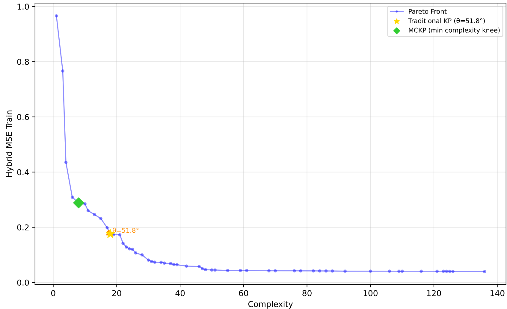
589_fri_c2_1000_25 - Run 28 - MVP - Hybrid MSE Train \lambda_1=0.00, \lambda_2=0.00, \lambda_3=0.00 | Difficulty: 1.00 | Method: hmr
