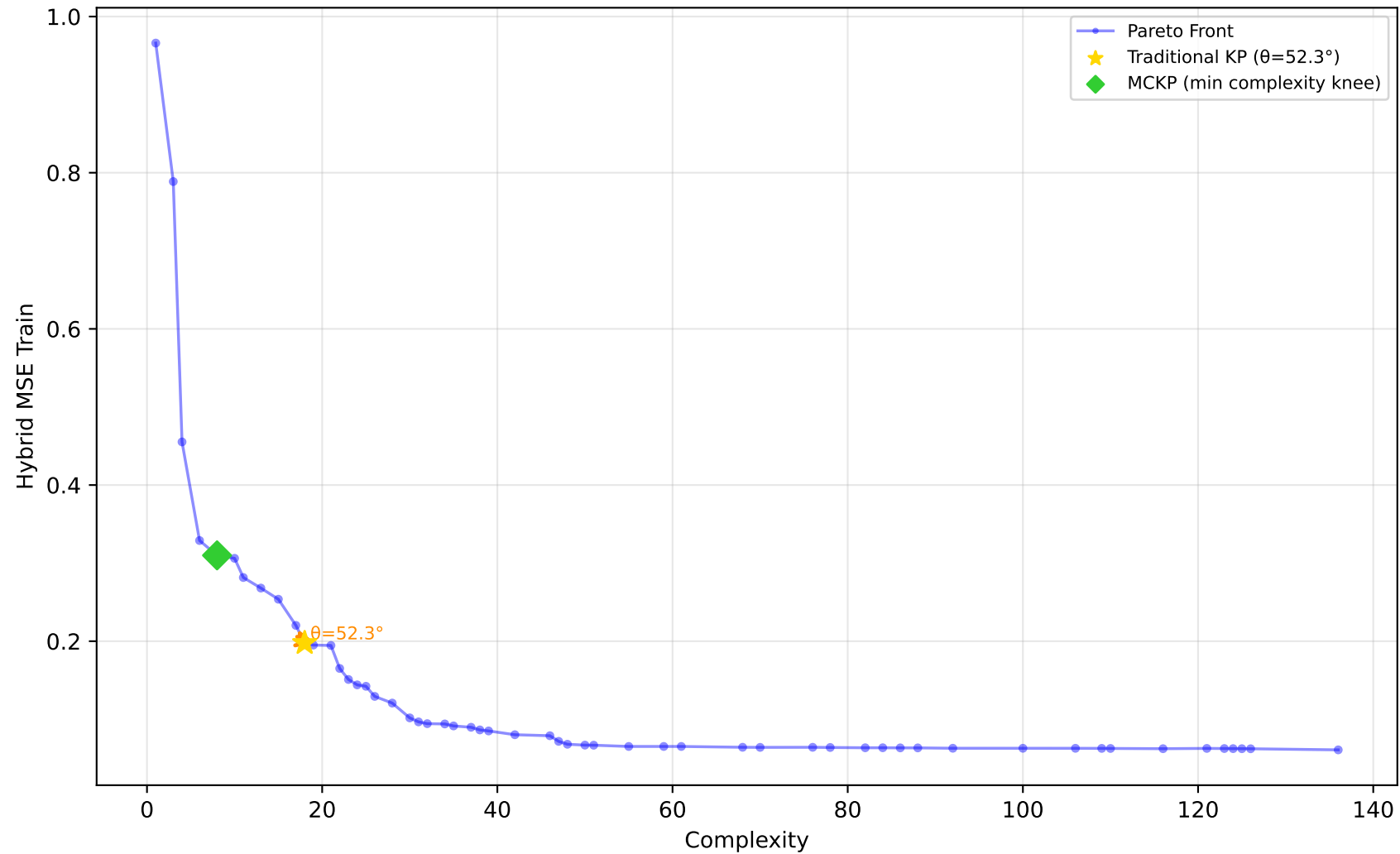
589_fri_c2_1000_25 - Run 28 - MVP - Hybrid MSE Train \lambda_1=0.30, \lambda_2=0.00, \lambda_3=0.20 | Difficulty: 1.00 | Method: hmr
