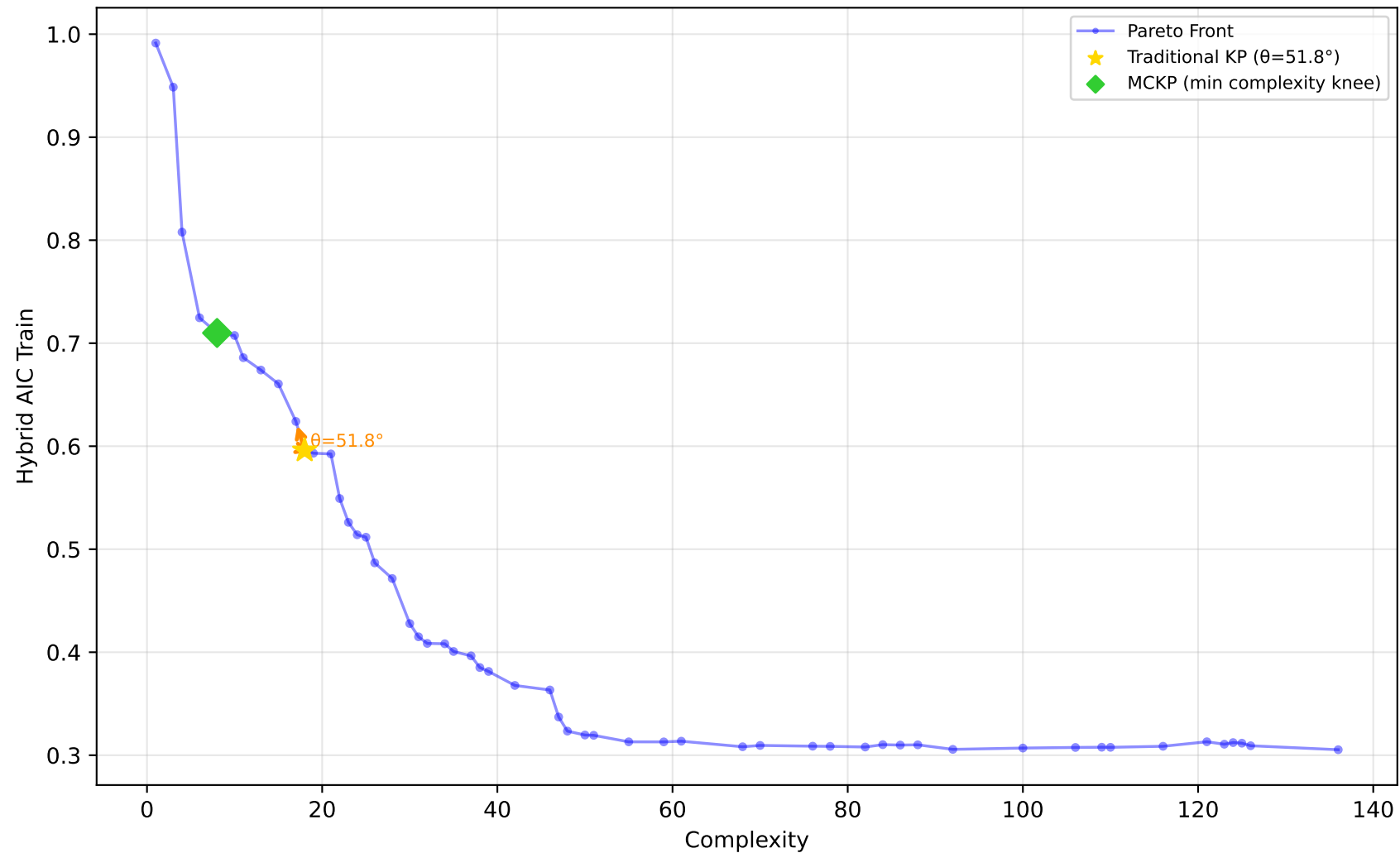
589_fri_c2_1000_25 - Run 28 - SVP - Hybrid AIC Train \lambda_1=0.20 , \bar{\lambda}_2=0.00 , \bar{\lambda}_3=1.00 | Difficulty: 1.00 | Method: hmr
