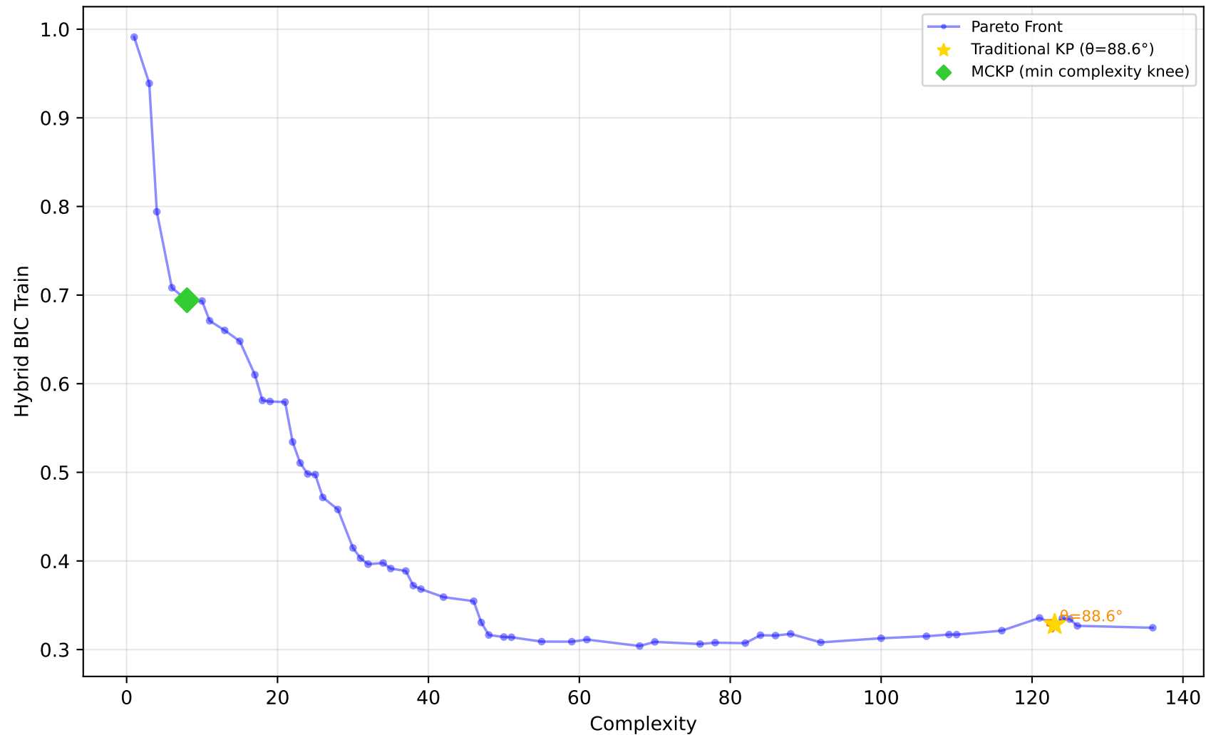
589_fri_c2_1000_25 - Run 28 - SVP - Hybrid BIC Train \lambda_1=0.10, \bar{\lambda}_2=0.00, \bar{\lambda}_3=0.10 | Difficulty: 1.00 | Method: hmr
