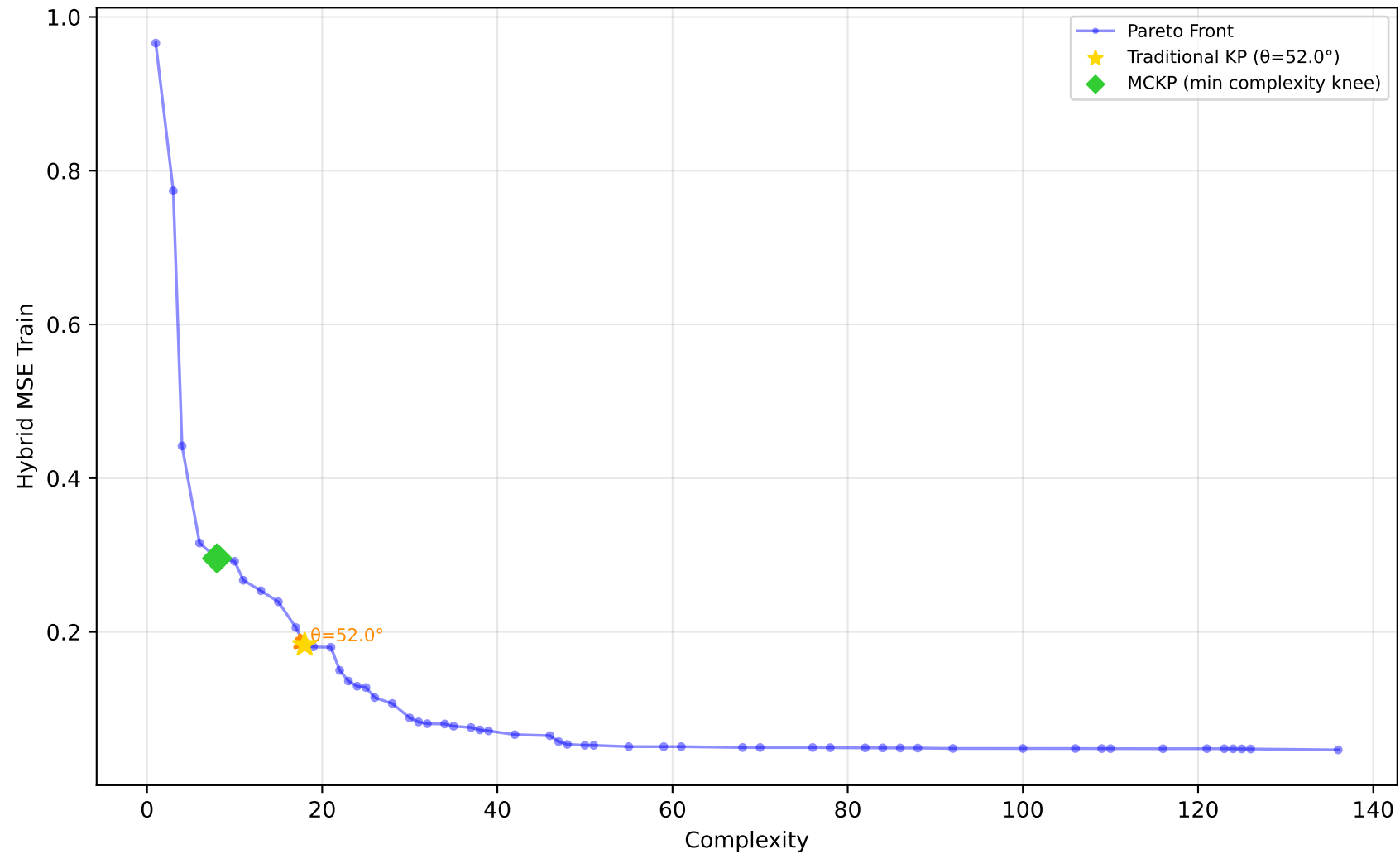
589_fri_c2_1000_25 - Run 28 - SVP - Hybrid MSE Train \lambda_1=0.10, \bar{\lambda}_2=0.00, \bar{\lambda}_3=0.10 | Difficulty: 1.00 | Method: hmr
