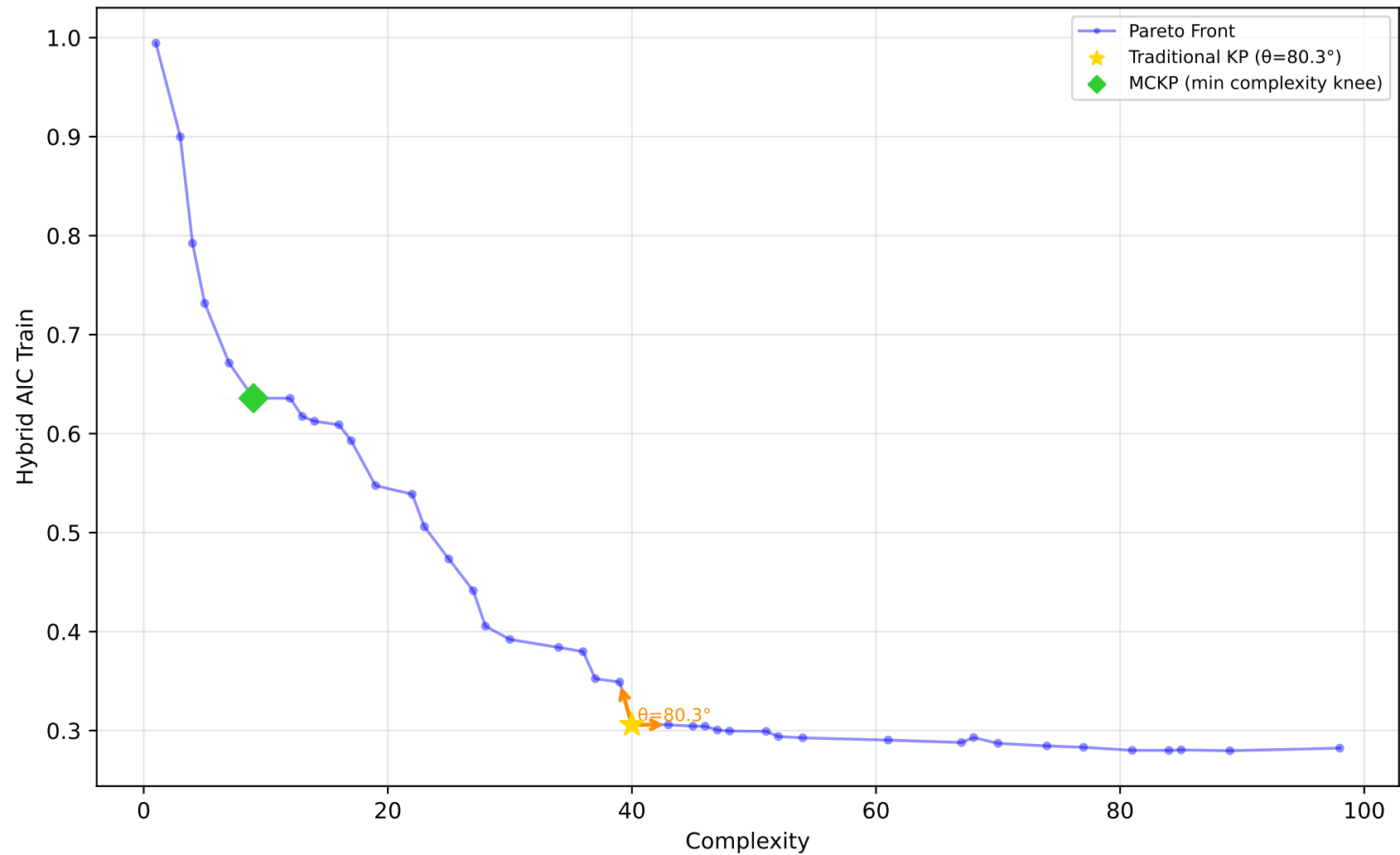
589_fri_c2_1000_25 - Run 29 - MVP - Hybrid AIC Train \lambda_1=0.00, \lambda_2=0.00, \lambda_3=0.00 | Difficulty: 1.00 | Method: hmr
