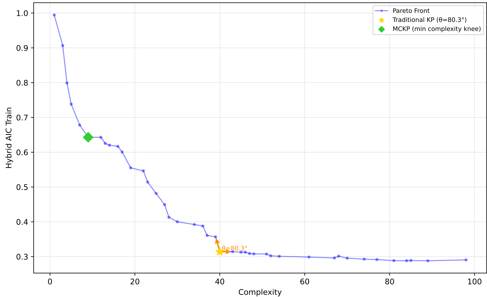
589_fri_c2_1000_25 - Run 29 - SVP - Hybrid AIC Train \lambda_1=0.10, \bar{\lambda}_2=0.00, \bar{\lambda}_3=0.10 | Difficulty: 1.00 | Method: hmr
