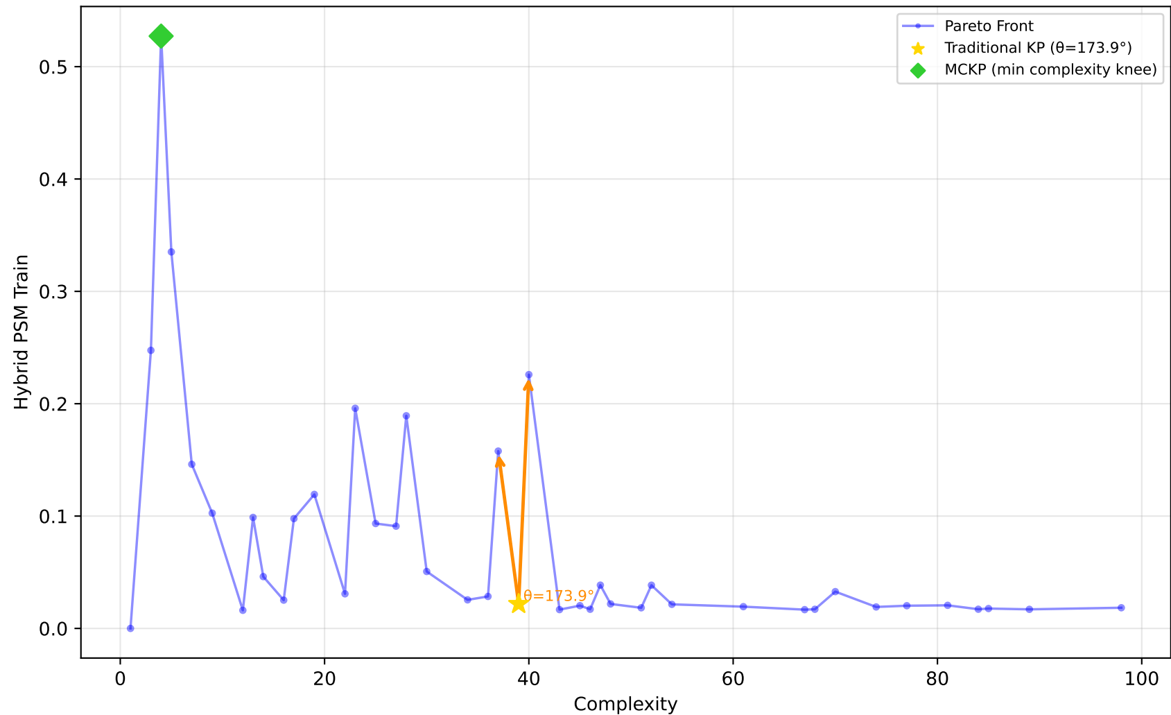
589_fri_c2_1000_25 - Run 29 - SVP - Hybrid PSM Train \lambda_1=0.20, \lambda_2=0.00, \lambda_3=1.00 | Difficulty: 1.00 | Method: hmr
