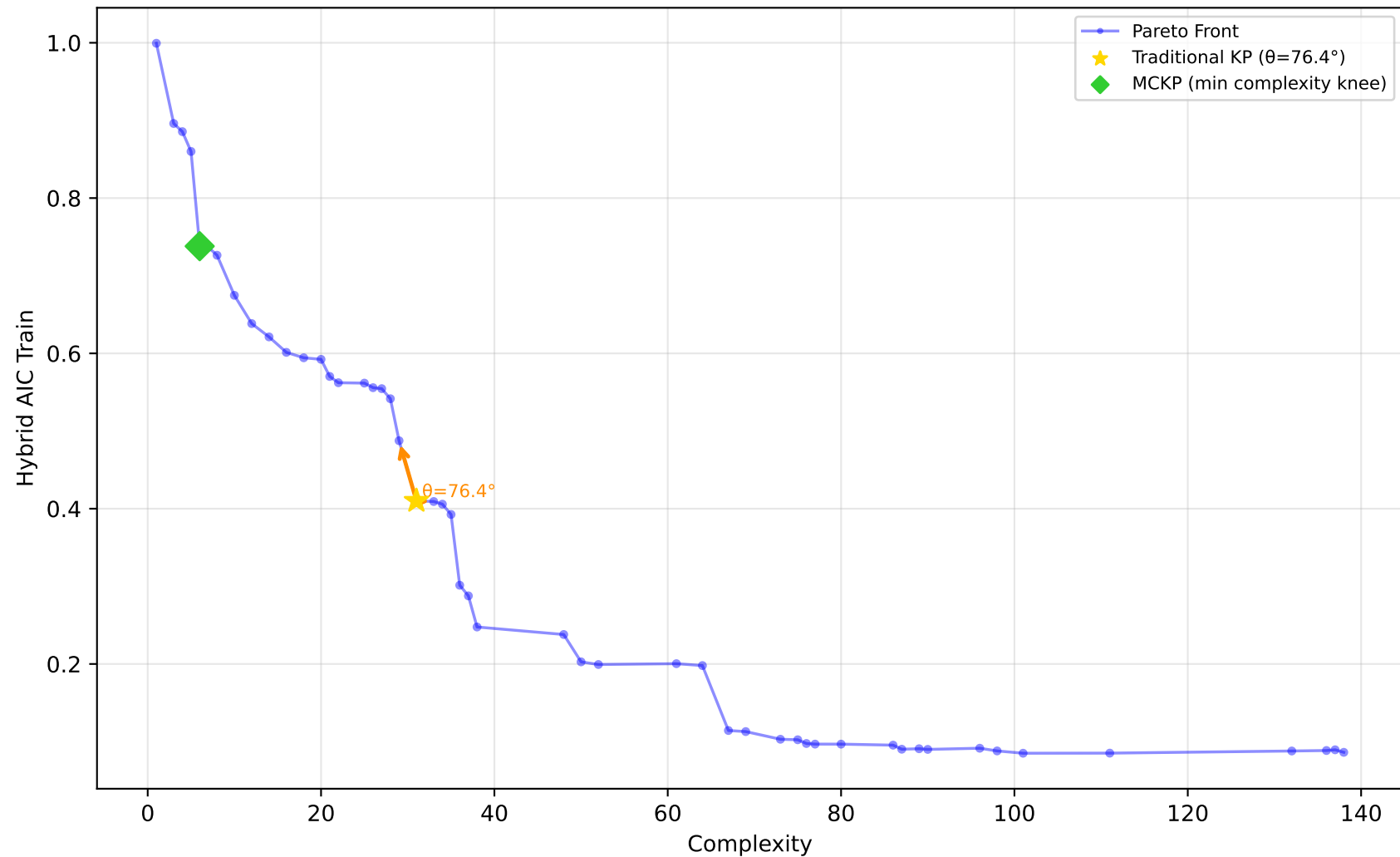
589_fri_c2_1000_25 - Run 2 - MVP - Hybrid AIC Train \lambda_1=0.00, \lambda_2=0.00, \lambda_3=0.00 | Difficulty: 1.00 | Method: hmr
